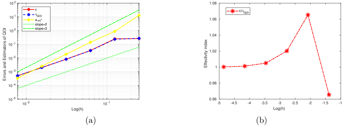
Figure 3: Diffusion problem, D = I_{\mathbb{R}^2} , regular solution. (a) : rates of convergence. (b) : effectivity index.
