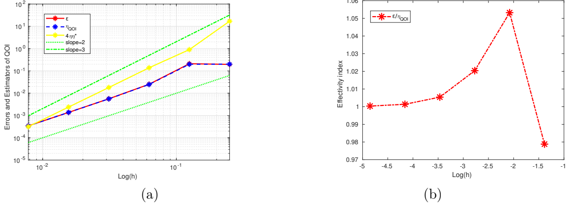
Figure 4: Diffusion problem, D(x, y) = (1+x^2+y^2)I_{\mathbb{R}^2} regular solution. (a) : rates of convergence. (b) : effectivity index.
