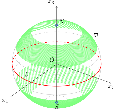
FIGURE 1. The equator \mathcal{E} (in red), a control region \bar{\omega} (in green), north and south pole (in blue).
