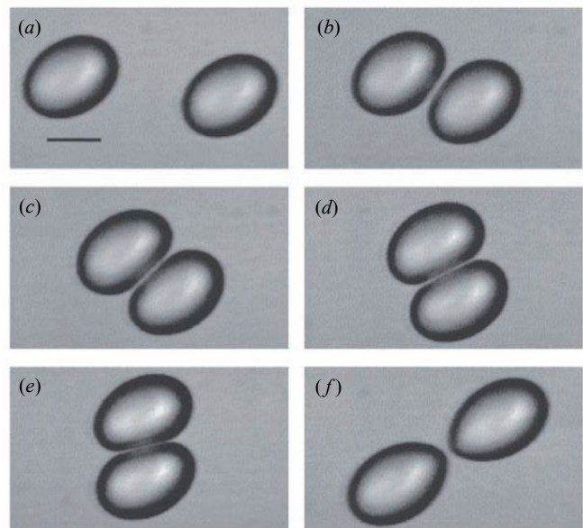
Figure 22. Successive snapshots of interacting drops with \lambda = 1.4 and R = 20 \mu\text{m} . The scale bar is 25 \mu\text{m} . Adapted from [209].
