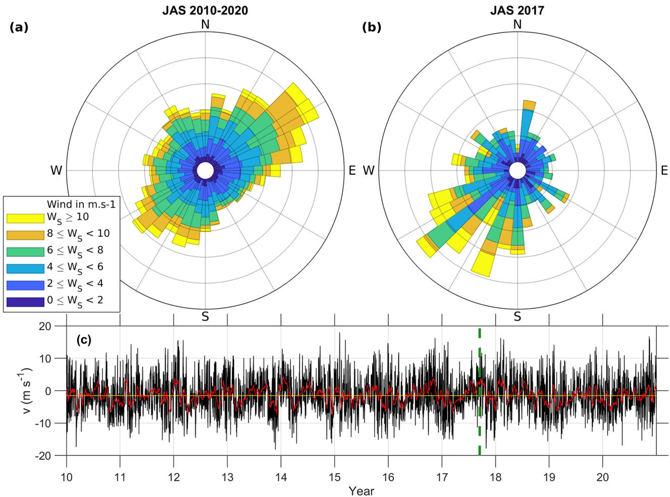
Figure 2. Wind rose diagrams of the wind speed ( W_s ) and direction north of Svalbard averaged over the box 80–80.7°N and 8–14°E. (a) Over July–August–September 2010–2020. (b) Over July–August–September 2017. (c) Meridional component of the wind at 10 m averaged in the same box over 2010–2020. The red line is a 20 days running mean. The yellow line is the meridional wind averaged over 2010–2020. The green dashed line indicates the glider mission in September 2017.
