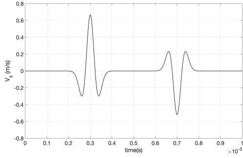
(a) The incident and reflected Ricker wavelet in the acoustic subdomain
