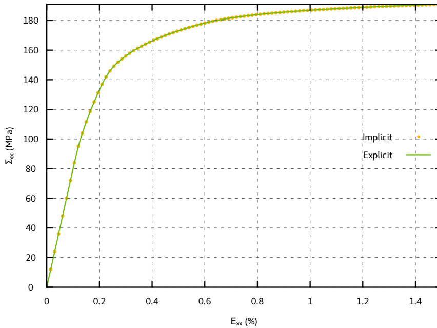
Figure 1: Comparison of the results of the implicit and explicit implementations respectively for a simple uniaxial tensile test
