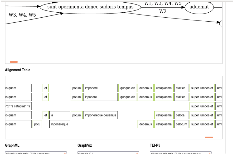
Figure 5: StemmaWeb.
