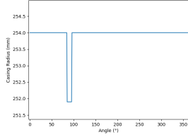
(c) Casing profile for 2 \leq t \leq 4
