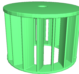
Fig. 13: Result of the marching cube method applied on the hexahedral mesh obtained from mesh S3, with l_{\max}=7 .
