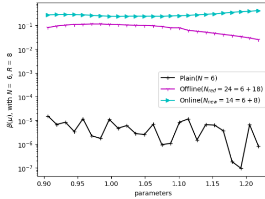
FIGURE 5 – Comparaison de \beta_{N,R}(\mu) .
