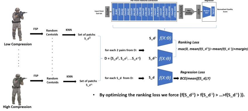
Fig. 1 : Training Process and model architecture.
