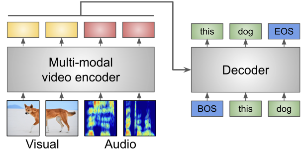
Figure 1: AVATAR : We propose a Seq2Seq architecture for audio-visual speech recognition. Our model is trained end-to-end from RGB pixels and spectrograms.
