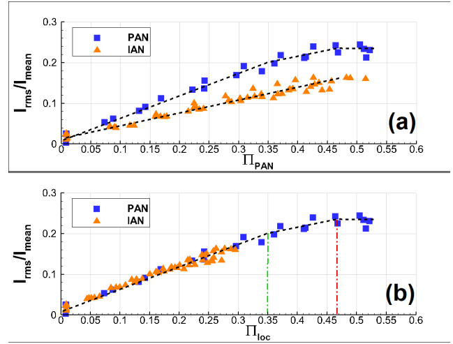
Figure 4. Flame response I_{rms}/I_{mean} for the central flame placed at PAN (blue squares) or IAN (orange triangles). (a) plot vs. acoustic amplitude at PAN \Pi_{ref} ; (b) plot vs. local acoustic amplitude \Pi_{loc} .
