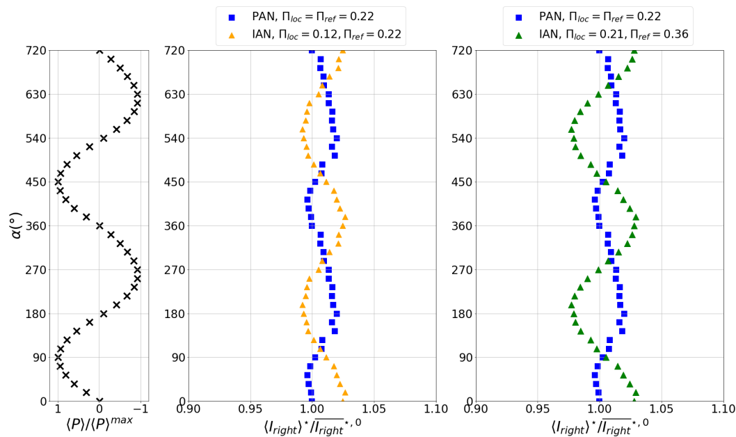
Figure 7. Evolution of the proportion of OH*-intensity in the right side of the injector axis reduced by the mean value without acoustics, \langle I_{right} \rangle^* / \overline{I_{right}^{*,0}} over a reconstructed acoustic pressure cycle, reproduced twice for the sake of clarity. Left: reconstructed acoustic pressure cycle; middle: \langle I_{right} \rangle^* / \overline{I_{right}^{*,0}} at PAN (blue squares) and at IAN (orange triangles) for similar values of \Pi_{ref} = 0.22 ; right: \langle I_{right} \rangle^* / \overline{I_{right}^{*,0}} at PAN (blue squares) and at IAN (green triangles) for similar values of \Pi_{loc} \simeq 0.22 .
