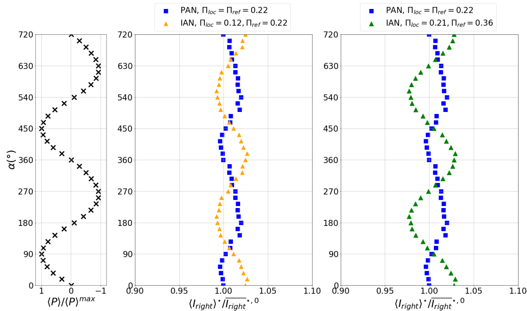
Figure 7. Evolution of the proportion of OH*-intensity in the right side of the injector axis reduced by the mean value without acoustics, \langle I_{right} \rangle^* / \overline{I_{right}^{*,0}} over a reconstructed acoustic pressure cycle, reproduced twice for the sake of clarity. Left: reconstructed acoustic pressure cycle; middle: \langle I_{right} \rangle^* / \overline{I_{right}^{*,0}} at PAN (blue squares) and at IAN (orange triangles) for similar values of \Pi_{ref} = 0.22 ; right: \langle I_{right} \rangle^* / \overline{I_{right}^{*,0}} at PAN (blue squares) and at IAN (green triangles) for similar values of \Pi_{loc} \simeq 0.22 .
