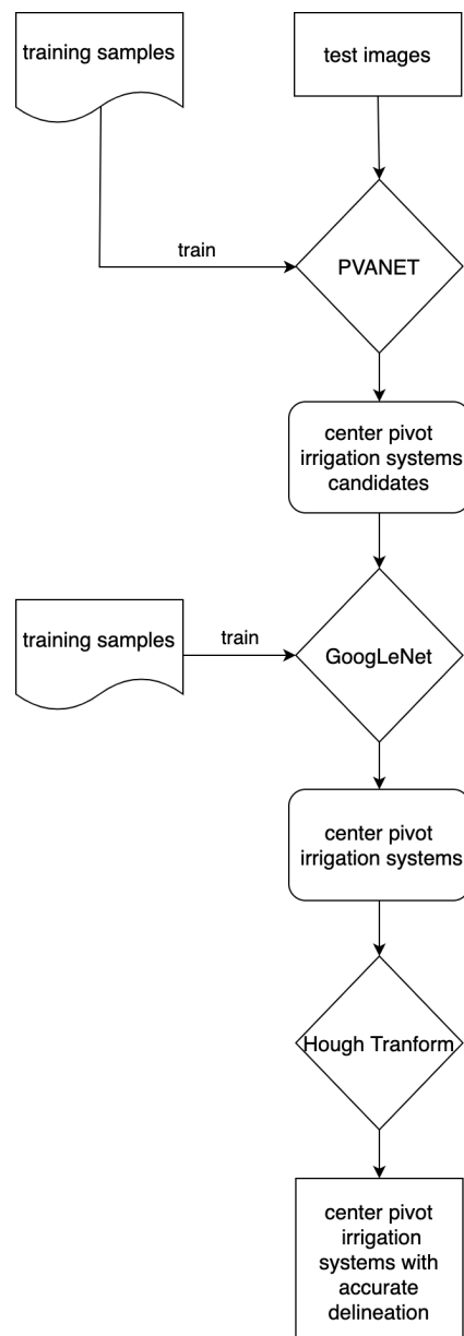
Figure 2. Flowchart of the proposed method.
