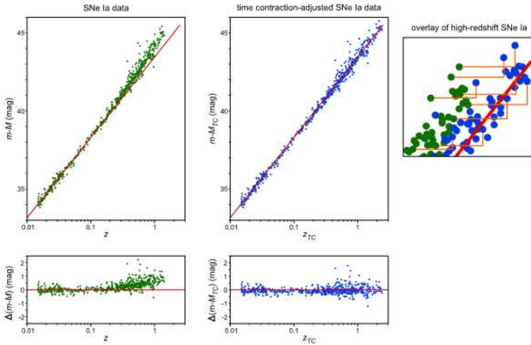
Fig. 1. Top: Diagrams of SNe plotted for z and m-M (green, left) and z_{TC} and m-M_{TC} for which redshifts and distance moduli have been adjusted to compensate for increased blueshifted emissions under TC conditions (blue, center). The straight line in each is a linear regression derived using SNe Ia with z < 0.14 . Bottom: Residuals in distance moduli relative to the linear regression line derived using SNe Ia with z < 0.14 . An overlay of high-redshift SNe Ia at increased magnification is shown on the right. Orange lines mark the shift between positions for selected SNe Ia.
