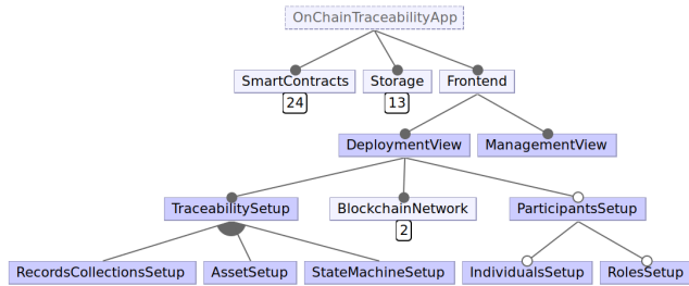
Figure 3: Frontend FM.
