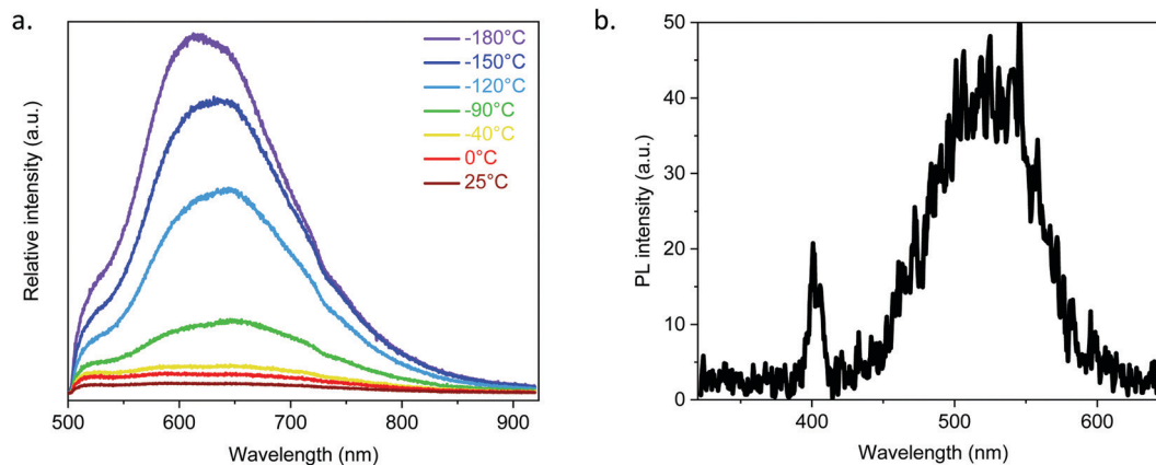
Fig. 3 Photophysical properties of [Ag_2(1,3-BDT)]_n : (a) temperature-dependent solid state emission spectra ( \lambda_{ex} = 410 nm) and (b) second harmonic generation response with incident beam at \lambda_{ex} = 800 nm and RT.
