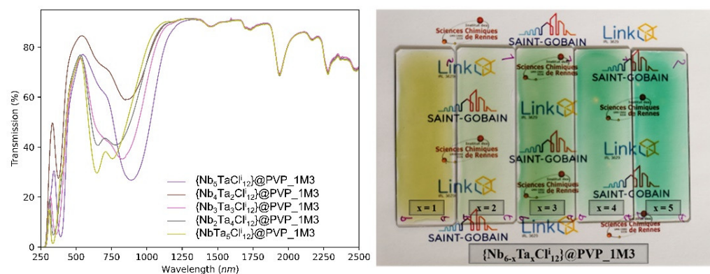
Figure 6. Camera image (right) and UV-Vis-NIR transmission spectra (left) of the \{\text{Nb}_{6-x}\text{Ta}_x\text{Cl}^{\text{i}}_{12}\}\text{-5@PVP} nanocomposite films deposited on glass substrates (sample sizes are 2.5 \text{ cm} \times 7.5 \text{ cm} ).
