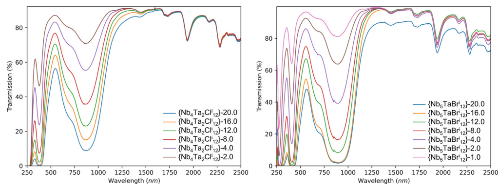
Figure 7. UV-Vis-NIR transmission spectra of the \{\text{Nb}_{6-x}\text{Ta}_x\text{X}_{12}\}\text{-Y@PVP} ( \text{X} = \text{Cl}, \text{Br}; x = 1, 2 ) nanocomposite films for concentrations ranging from 1 to 20 \text{g}\cdot\text{L}^{-1} .
