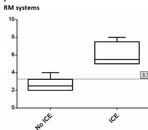
Fig. 6. Correlation between horizontal gene transfer and restriction modifications systems in M. agalactiae . (a) Number of restriction modification systems (RMtot), Type II RM systems (Type II), methylated motifs (Ndetected motifs), restriction endonucleases (REase), and mobile elements detected in the ten strains of M. agalactiae . The number of mobile elements includes CDS annotated by RAST (30) as mobile elements, integrases, transposases and prophage elements and genes identified by Blast against 5632 ICEA (e value less than to 10^{-3} ) as belonging to ICE elements. Based on previous work (59), elements were counted as ICE when at least the following three main components were present and complete: CDS5 and CDS17 encoding the conjugation factors TraE and TraG, respectively, and CDS22 encoding the integrase. (b) Boxplot showing the strong correlation between the presence of Type II active RM systems (excluding the 5'-GANTC-3' methylation found in all strains) and the number of mobile elements (Pearson's r=0.78 , P=0.008 ) in M. agalactiae genomes. (c) Boxplot showing the very strong correlation between the presence of ICE elements and the number of RM systems in M. agalactiae genomes (Pearson's r=0.86 , P=0.001 ). For both boxplots, the dotted line represents the median; their values are indicated in the grey box on the right.
