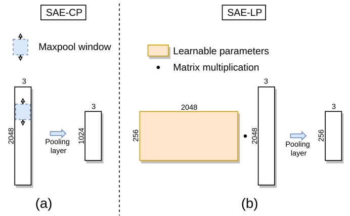
Fig. 5. Illustration of the two pooling methods used when downsampling 2048 frequencies. (a) - A classic pooling window of size 2 with stride 2 allows to reduce the resolution of the spectral coefficients by a factor of 2. This method is referred to Spectral Autoencoder with classic pooling (SAE-CP). (b) - the downsampled spectral coefficients are computed by multiplying them with a matrix containing learnable parameters. The downsampling factor is larger than with the classic pooling (see Section 5.2 for more information). This method is referred to Spectral Autoencoder with learned pooling (SAE-LP).
