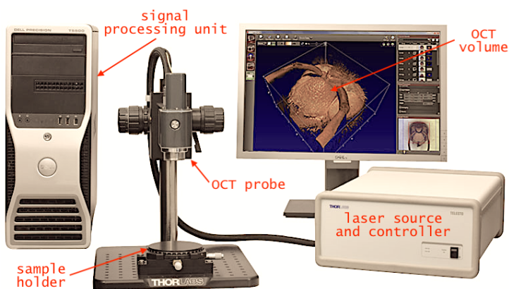
Figure 2: Photography of our OCT imaging system.
