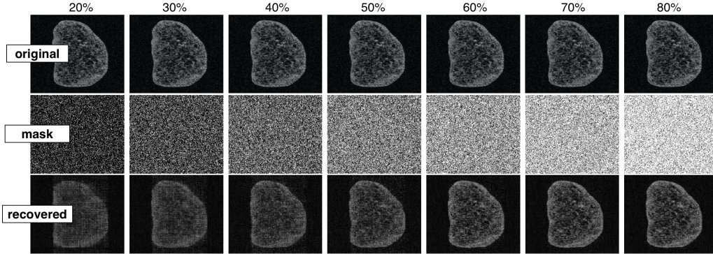
Figure 6: [sample: grape] - Reconstructed OCT images (only a 2D slice is shown in this example). First row corresponds to the original slice, second row the subsampled data (ranging from 20% to 80% with a step of 10%) to be reconstructed, and third row the reconstructed slices.
