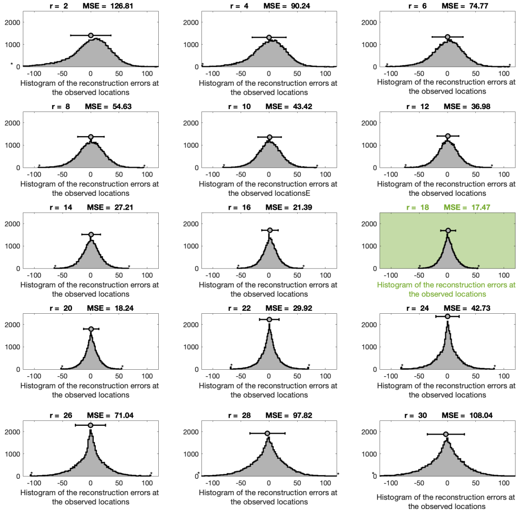
Figure 9: Histograms of the reconstructed error at the observed locations only. The plot in green shows the histogram associated with the smallest MSE over the total tensor image, corroborating the relevance of using histograms for accurate reconstruction.
