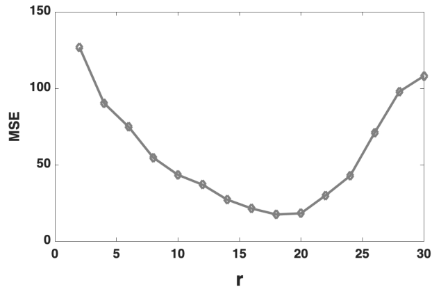
Figure 10: MSE over the whole reconstructed tensor image as a function of the rank
