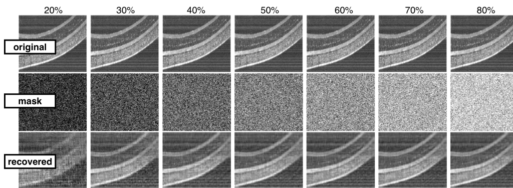
Figure 5: [sample: retina] - Reconstructed OCT images (only a 2D slice is shown in this example). First row corresponds to the original slice, second row the subsampled data (ranging from 20% to 80% with a step of 10%) to be reconstructed, and third row the reconstructed slices.
