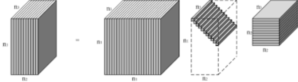
Figure 1: The t -SVD of a tensor
