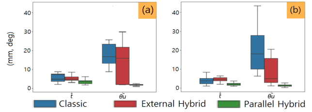
Fig. 3: Mean translation errors and rotation errors for the evaluated control laws. (a) tele-operation modes (b) comanipulation modes
