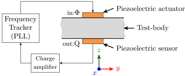
Figure 2: Frequency tracking principle: An harmonic excitation is send to the sensor test-body. Such electric potential excitation \Phi is transferred as vibrating force to the test-body by a piezoelectric actuator. The test-body response is then captured by a piezoelectric sensor in the form of electric charge Q . This charge is conditioned, and the sent to the tracking unit.
