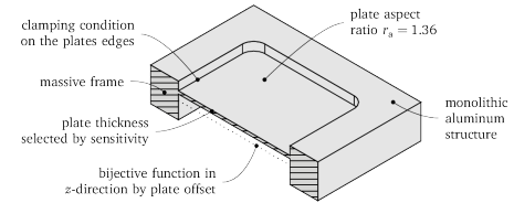
(a) Design parameters of the test-body plate
