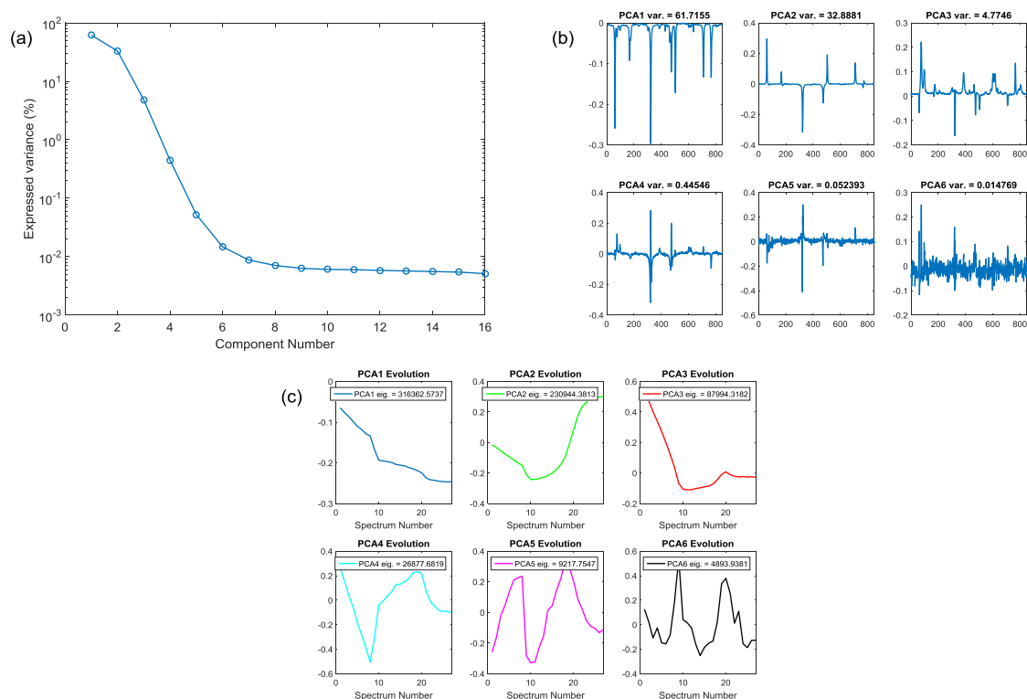
Figure S8: Variance plot (a), principal components (b) and the evolution of their contribution (c) along the full demagnesian-magnesian cycle of non-cubic Mg_2Pb .
