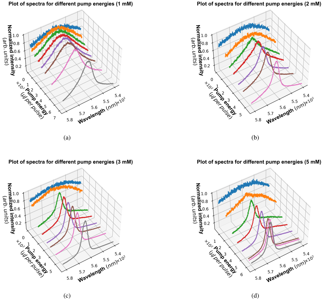
Figure 3: Emission spectra with different pump energy for gain concentrations 1 mM, 2 mM, 3 mM, 5 mM with 20 mg/ml scatterer concentration in (a), (b), (c), and (d) respectively.
