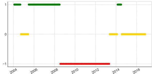
Figure 5: Unsupervised classification of the codings \mathbf{A}^{\text{Train}} in 3 clusters: \{-1 (red cross), 0 (yellow square), 1 (green dot) \} .
