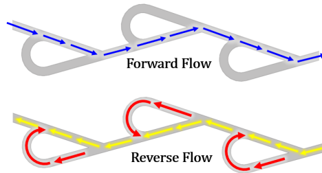
Fig. 1 Tesla valve flow behavior with low-resistance in forward direction (top) and high-resistance in reverse direction (bottom).
