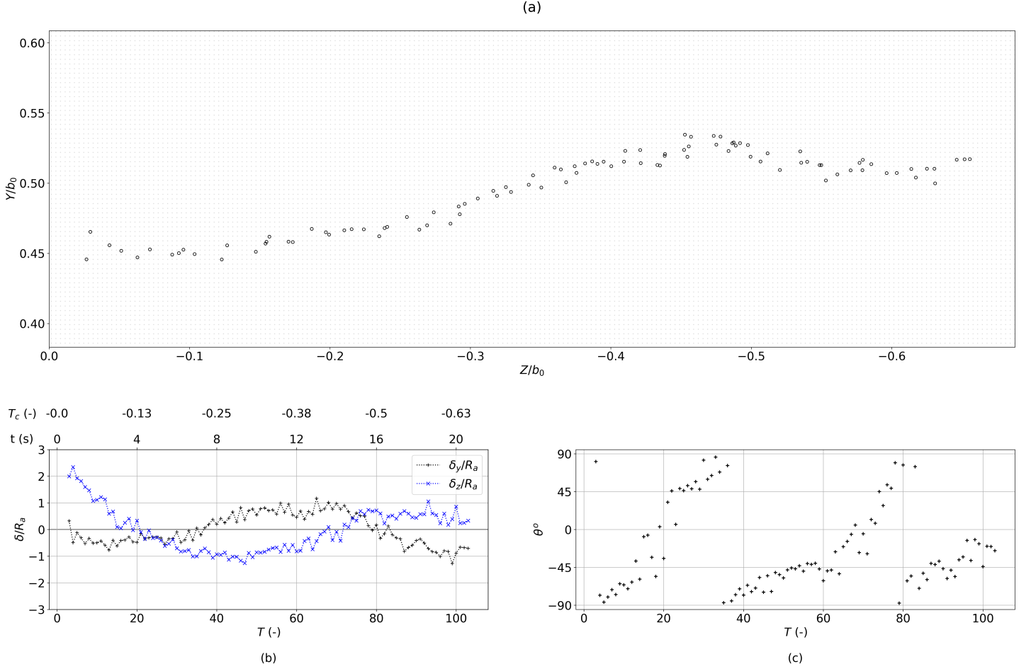
Fig. 9 Centroid trajectory \vec{x}_{\omega} for the vortices generated by the reference wing towed at U_0 = 2 m/s and \alpha = 3^\circ a) trajectory in the (y, z) -plane b) offset of \vec{x}_{\omega} with respect to the unperturbed trajectory as a function of time t , non-dimensional time T , and Crow time T_c . c) time evolution of the angle between the deformation and the horizontal plane.
