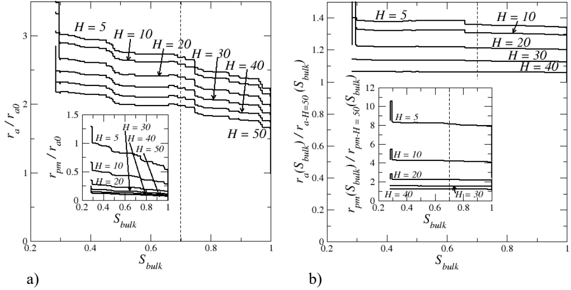
FIG. 17. a) Variation of the external mass transfer resistance and interfacial resistance (inset) with S_{bulk} for various external mass transfer layer thicknesses H ; r_{a0} = H/D_v is the external mass transfer resistance for the considered value of H at the very beginning of drying when the vapor partial pressure is spatially uniform at the surface; b) External mass transfer resistance rescaled by its value for H = 50 as a function of S_{bulk} . The inset shows the interfacial resistance rescaled by its value for H = 50 as a function of S_{bulk} . The vertical dashed lines correspond to S_{bulk} = 0.7 considered as the saturation range upper bound over which the comparison with the CM should be performed. Results are for one given realization of a 30 \times 30 \times 30 network.
