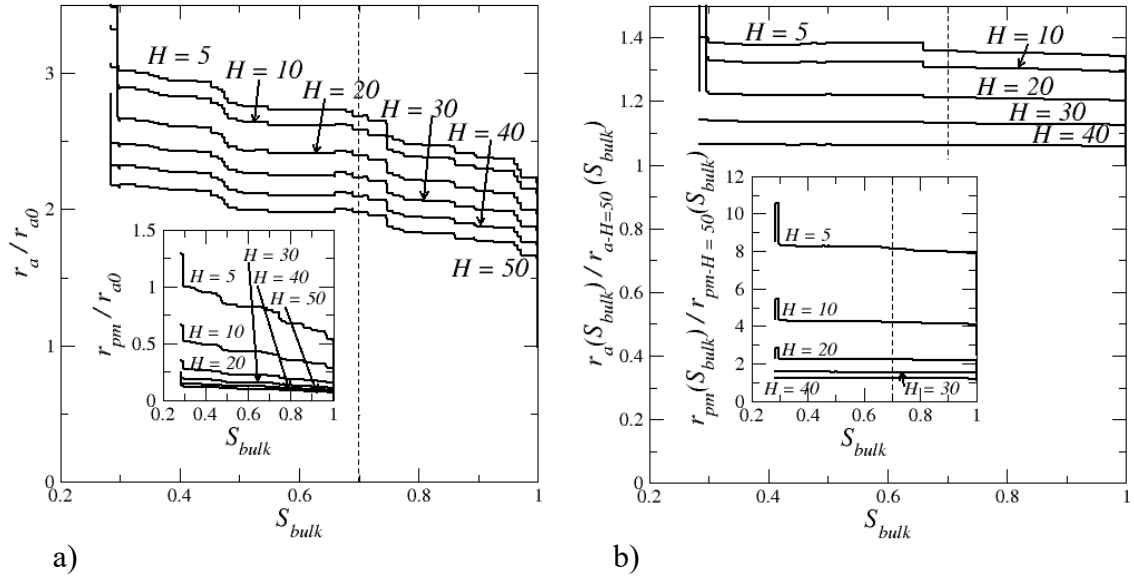
FIG. 17. a) Variation of the external mass transfer resistance and interfacial resistance (inset) with S_{bulk} for various external mass transfer layer thicknesses H ; r_{a0} = H/D_v is the external mass transfer resistance for the considered value of H at the very beginning of drying when the vapor partial pressure is spatially uniform at the surface; b) External mass transfer resistance rescaled by its value for H = 50 as a function of S_{bulk} . The inset shows the interfacial resistance rescaled by its value for H = 50 as a function of S_{bulk} . The vertical dashed lines correspond to S_{bulk} = 0.7 considered as the saturation range upper bound over which the comparison with the CM should be performed. Results are for one given realization of a 30 \times 30 \times 30 network.
