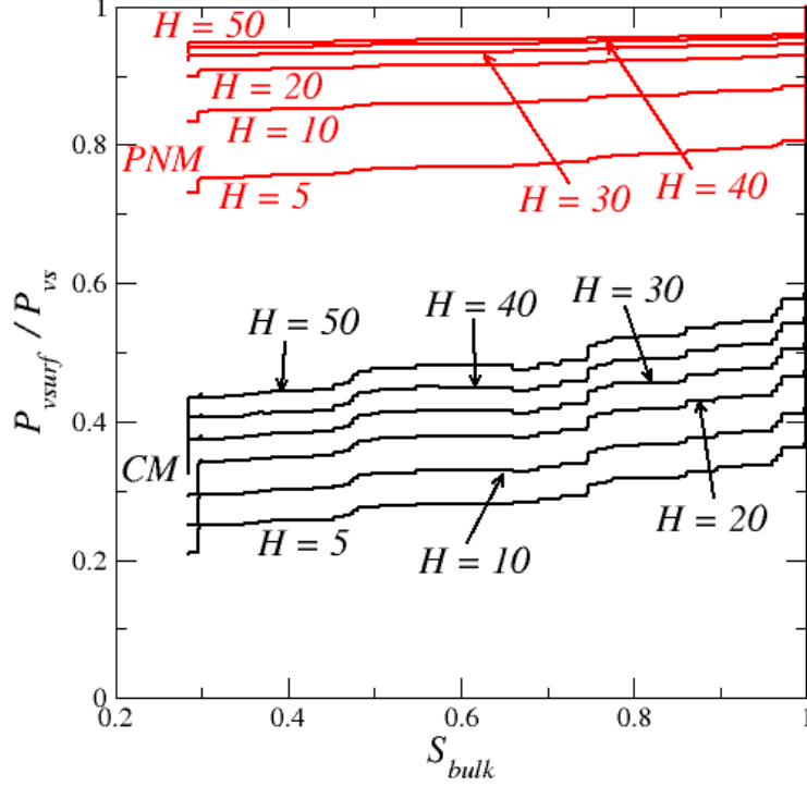
FIG. 14. Variation of the mean vapor partial pressure at the porous surface P_{vsurf} as a function of S_{bulk} for various external mass transfer layer thicknesses H with comparison with PNM results. The black curves ( CM ) are obtained using Eq.(23). Results are for one given realization of a 30 \times 30 \times 30 network.
