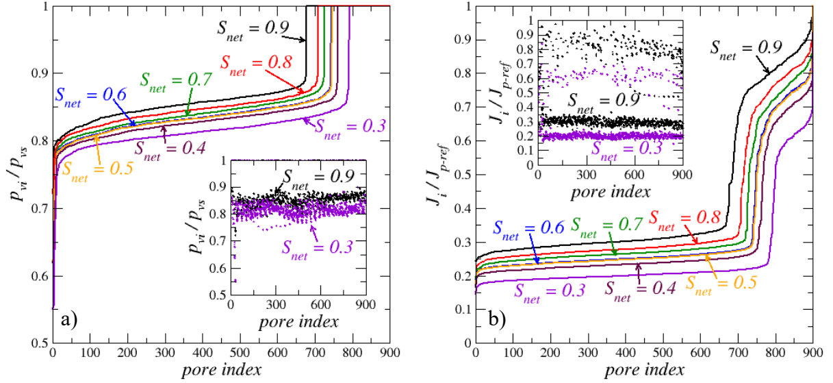
FIG. 16. a) Vapor partial pressure variations over the network top surface 900 pores for various overall network saturations. The vapor partial pressures are sorted in ascending order in the main figure. The inset shows the vapor partial pressure variations for two overall network saturations when the surface pores are scanned row by row; b) Evaporation rates from the 900 network top surface pores for various overall network saturations. The evaporation rates are sorted in ascending order in the main figure. The inset shows the evaporation rates for two overall network saturations when the surface pores are scanned row by row; J_{p-ref} = \frac{J_0}{N \times N} where J_0 is the evaporation rate when the network is fully liquid saturated. Results are for one given realization of a 30 \times 30 \times 30 network.
