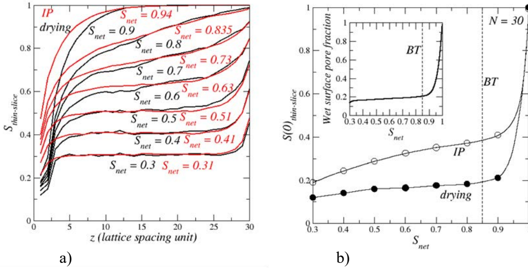
FIG.4. a) Saturation profiles in drainage and in drying according to IP algorithm and PNM drying algorithm, b) variation of saturation in the top slice in drying and in drainage (IP). The inset shows the variation of the fraction of pores at the surface filled with liquid. S_{net} is the network overall saturation. The IP profiles are average profiles over 50 realizations. The drying profiles are average profiles over 30 realizations.
