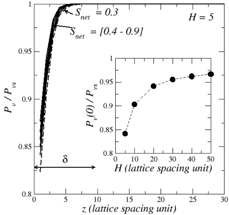
FIG. 9. Thin slice averaged vapor partial pressure profiles for one realization of the 30 \times 30 \times 30 network for S_{net} = 0.3, 0.4, 0.5, 0.6, 0.7, 0.8, 0.9 and H = 5 . The inset shows the variation of the thin slice averaged vapor partial pressure on top of network as a function of H for S_{net} = 0.4 .
