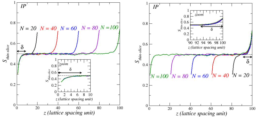
FIG. 7. Top and bottom edge effect region size. IP thin slice averaged saturation profiles for S_{net} = 0.5 for various network sizes. The inset in the figure on the left shows a zoom over the top region. The figure on the right shows the overlap of the profiles for the various network sizes in the bottom region. The inset in the figure on the right shows a zoom over the bottom region. Profiles are averaged profiles over 100 ( N=20 ), 80 ( N=40 ), 60 ( N=50 ), 30 ( N=80 ), 20 ( N=100 ) realizations, respectively
