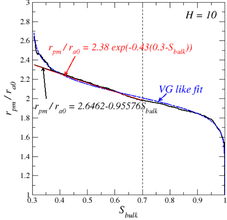
FIG. 11. Interfacial resistance as a function of S_{bulk} . The thick black curve is obtained from Eq.(13) and corresponds to the average over 50 realizations of the 30 \times 30 \times 30 network. The thin black line corresponds a linear fit over the range of saturation [0.4 -0.7]. The VG blue curve is obtained adjusting the parameters of a Van-Genuchten like expression (see text and Eq.(16)). The dashed line marks the saturation below which the comparison between the PNM simulations and the continuum models is considered as meaningful (see text).
