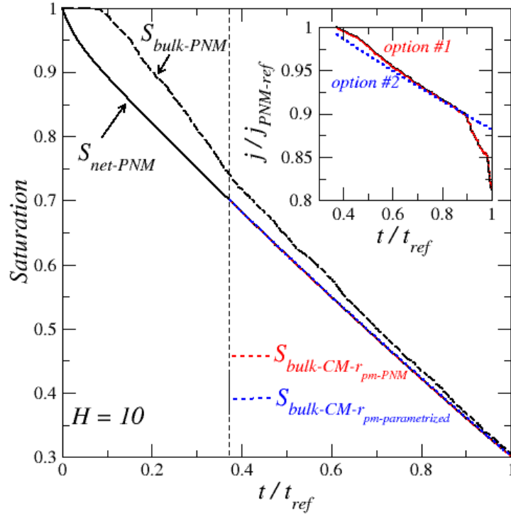
FIG.13. Variation of S_{bulk} as a function of time during stage 1. Comparison between the PNM data (averages over 50 realizations of the 30 \times 30 \times 30 network) and the results from the continuum model. The comparison is performed for overall saturations lower than 0.7 (part of the figure on the right side of the vertical dashed line) for the comparison not to be hampered by the initial significant finite size effect associated with the BT period (see text). The reference time is the time at the end of stage 1. The inset shows the variation of the evaporation flux for the two considered options (see text).
