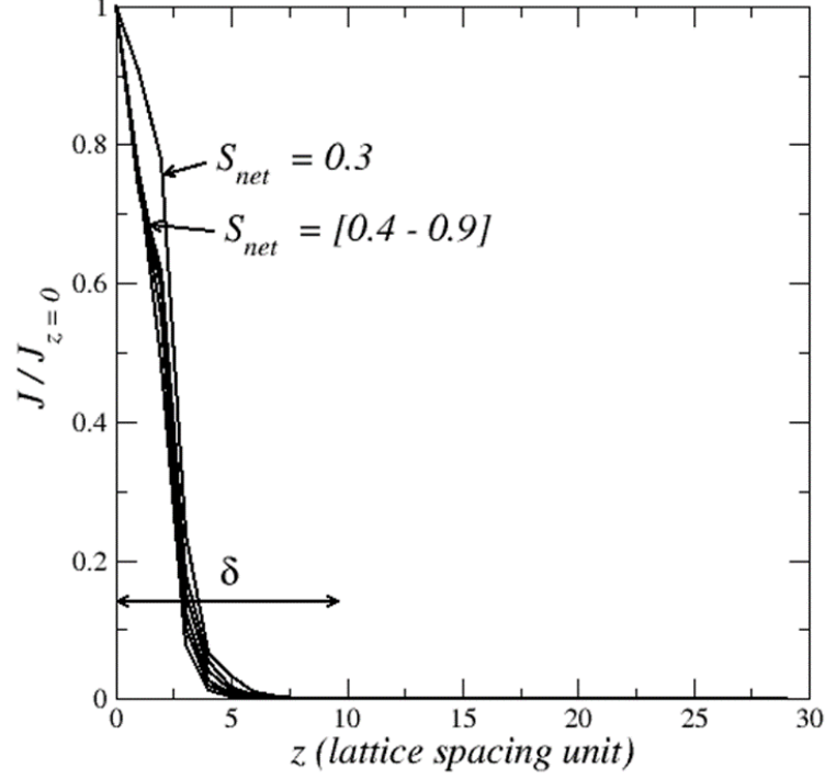
FIG. 12. Distribution of vapor diffusive flux over the top edge effect region from PNM simulations. Results are for one given realization of the 30 \times 30 \times 30 network.
