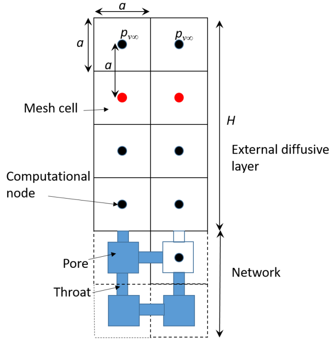
FIG. A1. Schematic of network and external mass transfer layer.
