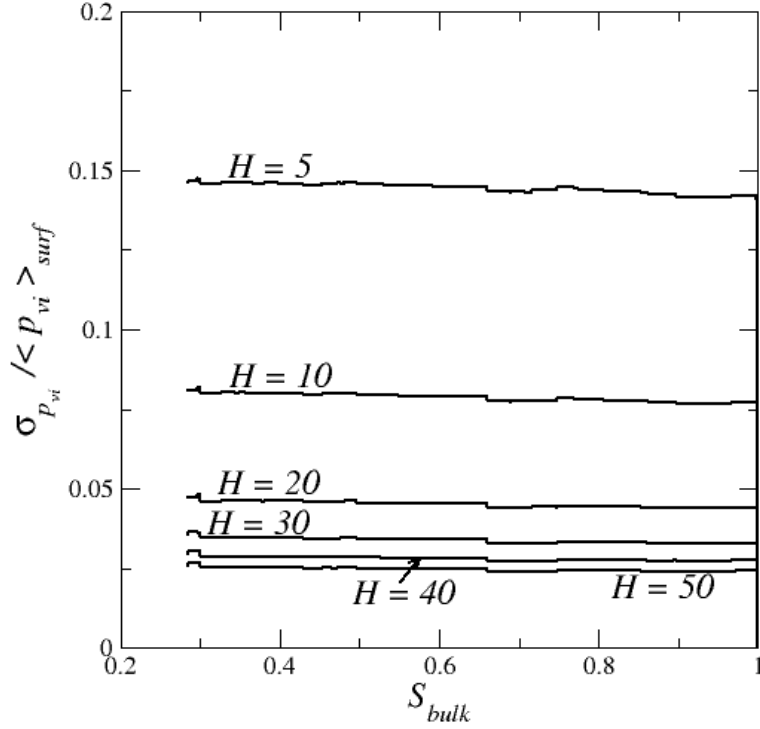
FIG.15. Standard deviation of the vapor partial pressure distribution at the surface as a function of S_{bulk} for various mass transfer external layer thicknesses. Results are for one given realization of the 30 \times 30 \times 30 network.
