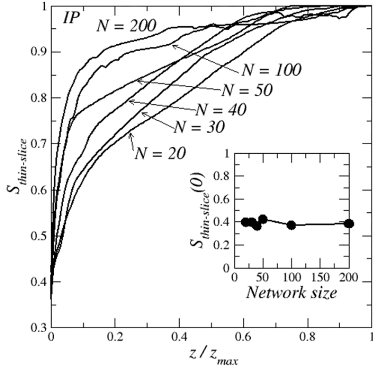
FIG. 6. IP saturation profiles at breakthrough for various network sizes. The inset shows the saturation at network top in the first slice ( z = 0 ) as a function of network size. Profiles are averaged profiles over 150 ( N = 20 ), 100 ( N=30 ), 80 ( N=40 ), 60 ( N=50 ), 30 ( N=100 ), 10 ( N=200 ) realizations, respectively
