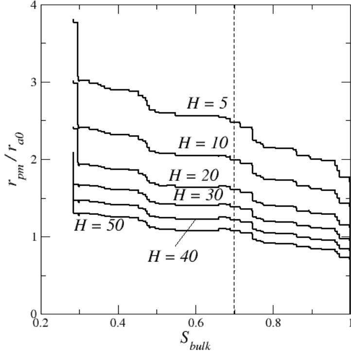
FIG. 10. Interfacial resistance from Eq.(13) as a function of S_{bulk} for various external mass transfer layer thicknesses H . Results are for one realization of the 30 \times 30 \times 30 network.
