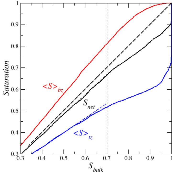
FIG. A2. Mean saturation S >_{tz} in the top edge effect region, mean saturation in the bottom edge effect region S >_{bz} and overall network saturation S_{net} as a function of the saturation in the bulk. These results are averages considering 200 realizations of the 30 \times 30 \times 30 network ( S >_{bz} from IP simulations) or 50 realizations ( S >_{tz} using the drying PNM algorithm) respectively.
