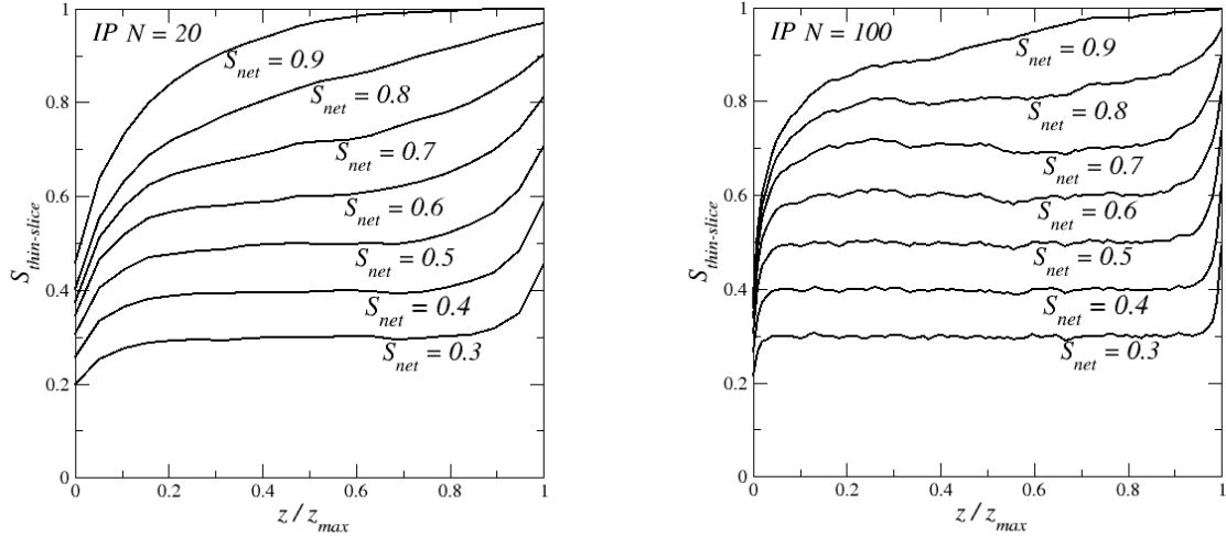
FIG.5. IP thin slice averaged saturation profiles for S_{net} = 0.3, 0.4, 0.5, 0.6, 0.7, 0.8, 0.9 and N = 20 (averaged over 100 realizations) and N = 100 (averaged over 20 realizations). The overall saturation at breakthrough is S_{net} \approx 0.83 for N = 20 and S_{net} \approx 0.92 for N = 100 .
