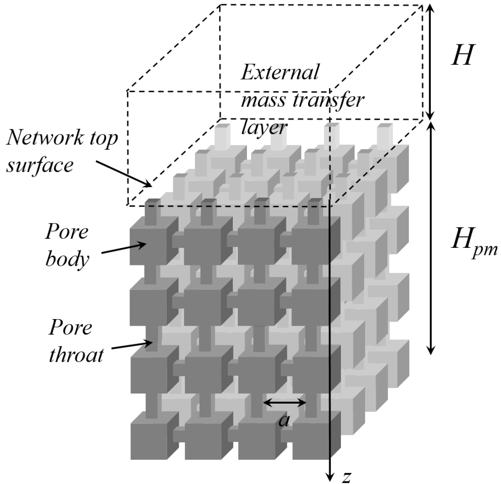
FIG.2. Sketch of pore network model with external mass transfer layer on top.
