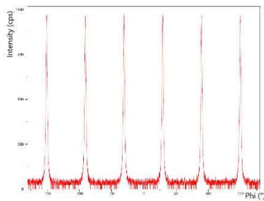
Fig. 2. \phi -scan \text{LiNbO}_3 c-sapphire heterostructure grown at 0.2 mbar, 600°C, \text{LiNbO}_3 target performed on \text{LiNbO}_3 (0 0 6).
