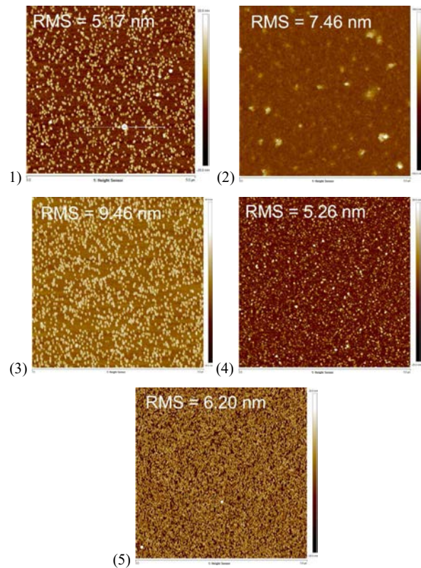
Fig. 7. AFM micrographs of \text{LiNbO}_3 films deposited on a\text{-Al}_2\text{O}_3 substrates grown at: (1) 0.2 mbar, 500°C, \text{LiNbO}_3 target; (2) 0.007 mbar, 500°C, \text{LiNbO}_3 target; (3) 0.2 mbar, 600°C, \text{LiNbO}_3 target; (4) 0.2 mbar, 600°C, \text{Li}+\text{LiNbO}_3 target; (5) 0.007 mbar, 500°C, \text{Li}+\text{LiNbO}_3 target. Scan size: (5 \times 5) \mu\text{m}^2 .
