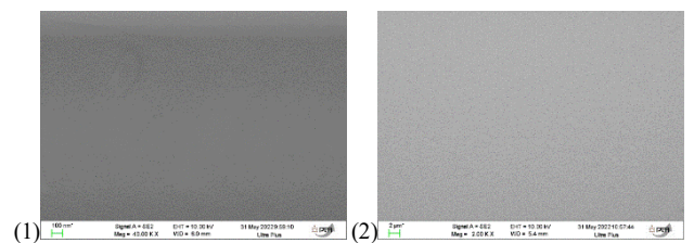
Fig. 4. SEM micrographs of \text{LiNbO}_3 c- \text{Al}_2\text{O}_3 heterostructures grown at: (1) 0.2 mbar, 500°C, \text{LiNbO}_3 target; (2) 0.2 mbar, 600°C, \text{LiNbO}_3 target.
