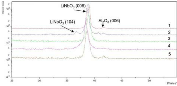
Fig. 1. \theta/2\theta XRD pattern of the \text{LiNbO}_3 c-sapphire heterostructure grown at: (1) 0.2 mbar, 500°C, \text{LiNbO}_3 target; (2) 0.007 mbar, 500°C, \text{LiNbO}_3 target; (3) 0.2 mbar, 600°C, \text{LiNbO}_3 target; (4) 0.2 mbar, 600°C, \text{Li}+\text{LiNbO}_3 target; (5) 0.007 mbar, 500°C, \text{Li}+\text{LiNbO}_3 target.
