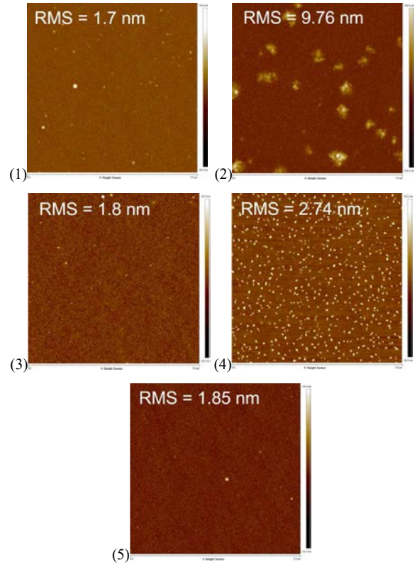
Fig. 3. AFM micrographs of \text{LiNbO}_3 films deposited on c- \text{Al}_2\text{O}_3 substrates grown at different conditions: (1) 0.2 mbar, 500°C, \text{LiNbO}_3 target; (2) 0.007 mbar, 500°C, \text{LiNbO}_3 target; (3) 0.2 mbar, 600°C, \text{LiNbO}_3 target; (4) 0.2 mbar, 600°C, \text{Li}+\text{LiNbO}_3 target; (5) 0.007 mbar, 500°C, \text{Li}+\text{LiNbO}_3 target. Scan size: (5 \times 5) \mu\text{m}^2 .
