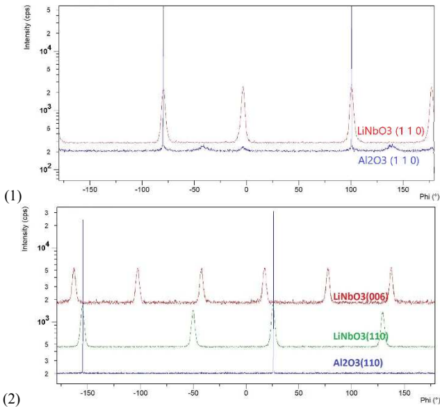
Fig. 6. \phi -scans of the \text{LiNbO}_3 a -sapphire heterostructures grown with \text{Li}+\text{LiNbO}_3 target at: (1) 0.2 mbar, 600°C; (2) 0.007 mbar, 500°C.
