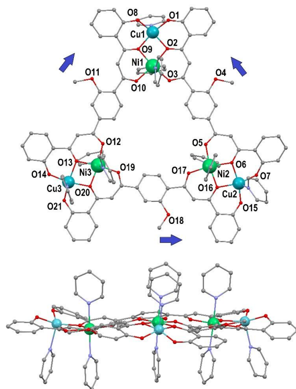
Figure 2. Two views of the structure of [Ni_3Cu_3(L)_3(py)_9] ( 1 ) with non-C and N atoms labelled, the top one showing with arrows the orientation of the -OMe groups that render each [NiCu] fragment inequivalent. H atoms not shown.
