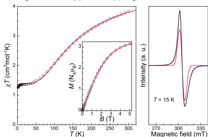
Figure 3. Left: \chi T vs. T plot of [\text{Ni}_3\text{Cu}_3(\text{L})_3(\text{py})_3] ( 1 ). The solid line is a fit (see text) to the experimental data (black circles) collected under a field of 0.5 T. Inset: magnetization vs. field data measured at 2 K. The red line is the Brillouin function at this temperature for a spin 1/2 with g = 2.20 . Right: CW-EPR spectrum obtained at X-band (9.418 MHz) and T = 15 K for a polycrystalline sample of 1 . The red line is the spectrum calculated with Easyspin 27 for S = 1/2 , g_{\text{eff}} = 2.206 and 6.5 mT Gaussian line broadening.
