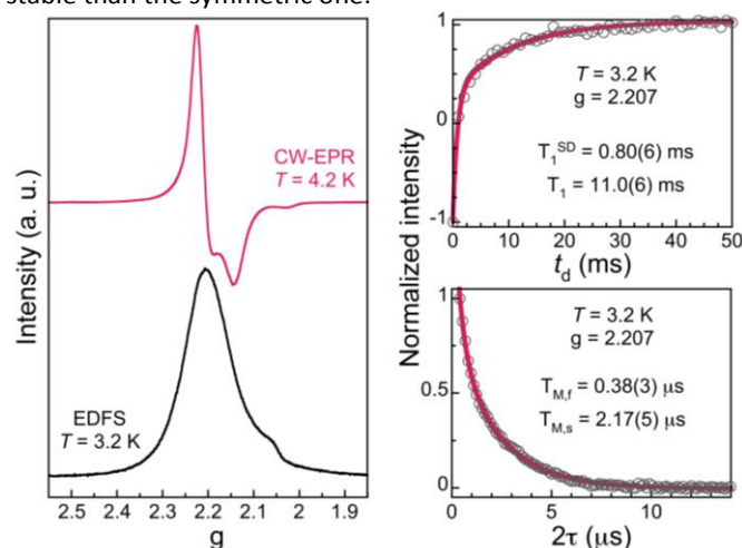
Figure 4. (Left) Frozen solution CW (top, X band) and echo detected (bottom, Q band) EPR of 1 at the indicated temperatures. (Right) Inversion recovery (top) and Hahn-echo decay (bottom) of the spin resonance of 1 (see legend).
