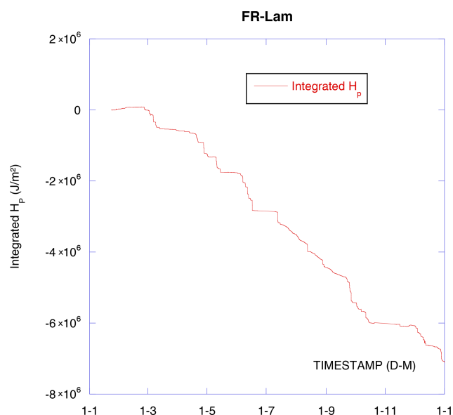
Figure 7. Integrated rainfall cooling H_p .
