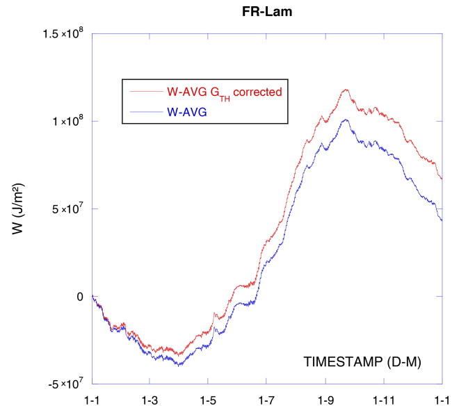
Figure 9. Integrated, averaged (among the plates), measured soil heat flux: W-AVG and the same integrated flux with geothermal effect subtracted: W-AVG G_{TH} corrected.
