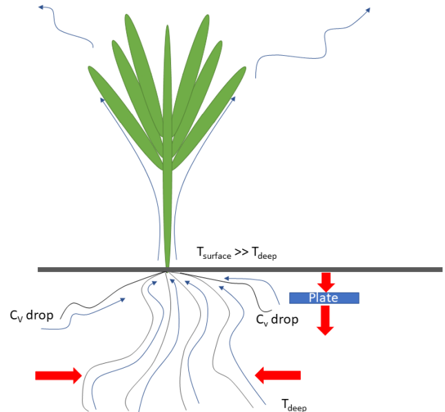
Figure 5. Root-absorbed water flows up from the deep soil at low temperature to the hot sun-heated soil surface, provoking a heat transfer between the soil and the roots. Shallow roots absorb water, drying soil and lowering its volumetric heat capacity C_v . Water is stored, and then energy is evacuated from the soil.
