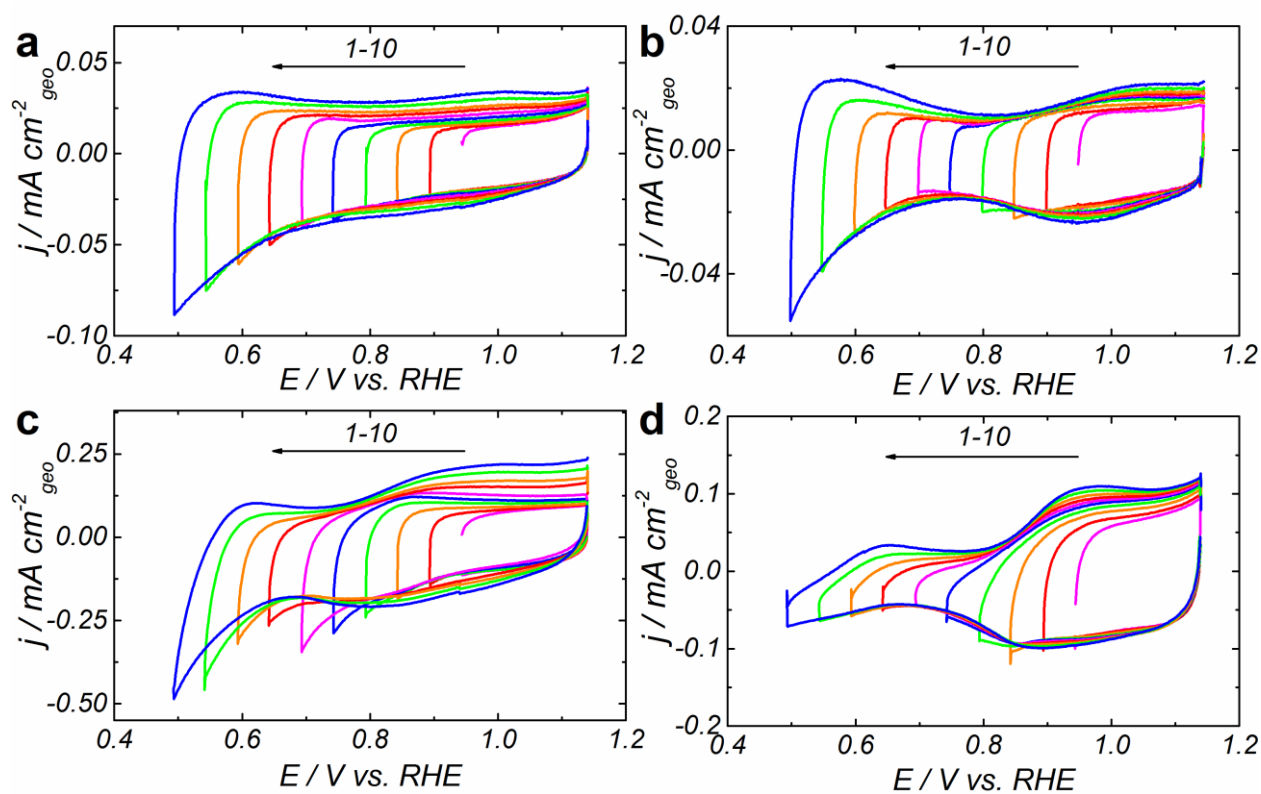
Figure 4. Experimental CVs with decreasing cathodic potential limit for GC-supported thin films of oxide/carbon composites in N 2 -purged 1 M NaOH at 10 mV s -1 for LaMnO 3 (a), Mn 2 O 3 _milled (b), MnO 2 (c), and MnOOH (d). Currents are normalized to the geometric area of the electrode, and corrected to the background currents measured on Sibunit carbon under the same conditions.
