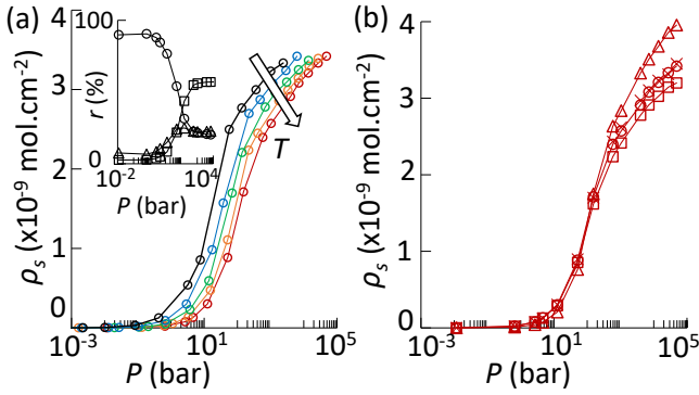
Figure 4: (color online) (a) Adsorption isotherms for methane at the external surface of the zeolite layer a (these data are obtained for the surface model s1 in which surface atoms are frozen). Different colors correspond to the following temperatures: 300 K (red), 275 K (orange), 250 K (green), 225 K (blue), 200 K (black). The methane adsorbed amounts are expressed as surface densities \rho_s in \text{mol}\cdot\text{cm}^{-2} . The insert shows the following ratios at 300 K where N is the total number of methane in the system: methane at the surface N_s/N (line with open triangles), methane inside the core N_c/N (line with open circles), methane in the external phase N_e/N (line with open squares). (b) Adsorption isotherms for methane at the external surface for layers a , b , c which correspond to the lines with open circles, open squares, and open triangles, respectively. The symbols are obtained for the surface model s1 in which surface atoms are frozen (s1 model). The crosses correspond to data for the layer a with the flexible surface model (s2 model). Note that the data for the s1 and s2 models are nearly identical.
