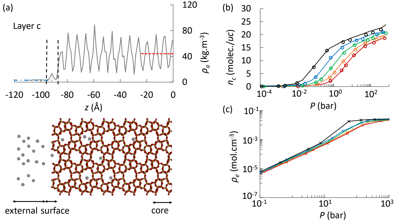
Figure 3: (color online) (a) Methane density for the silicalite-1 layer aligned along the c crystallographic axis. For visualization purpose, only the left side of the layer is shown (the system is symmetrical with respect to the position z = 0 ). The cavity size is about 1/3 of the Lennard-Jones size parameter for the methane molecule. (b) and (c) show the adsorption isotherms in the core of the zeolite layer and density in the external fluid phase, respectively. Different colors correspond to different temperatures T : 300 K (red), 275 K (orange), 250 K (green), 225 K (blue), 200 K (black). In (b), the lines show the adsorbed amounts obtained for the infinite zeolite while the open circles show the adsorbed amounts obtained by counting methane molecules adsorbed in the core of the layers.
