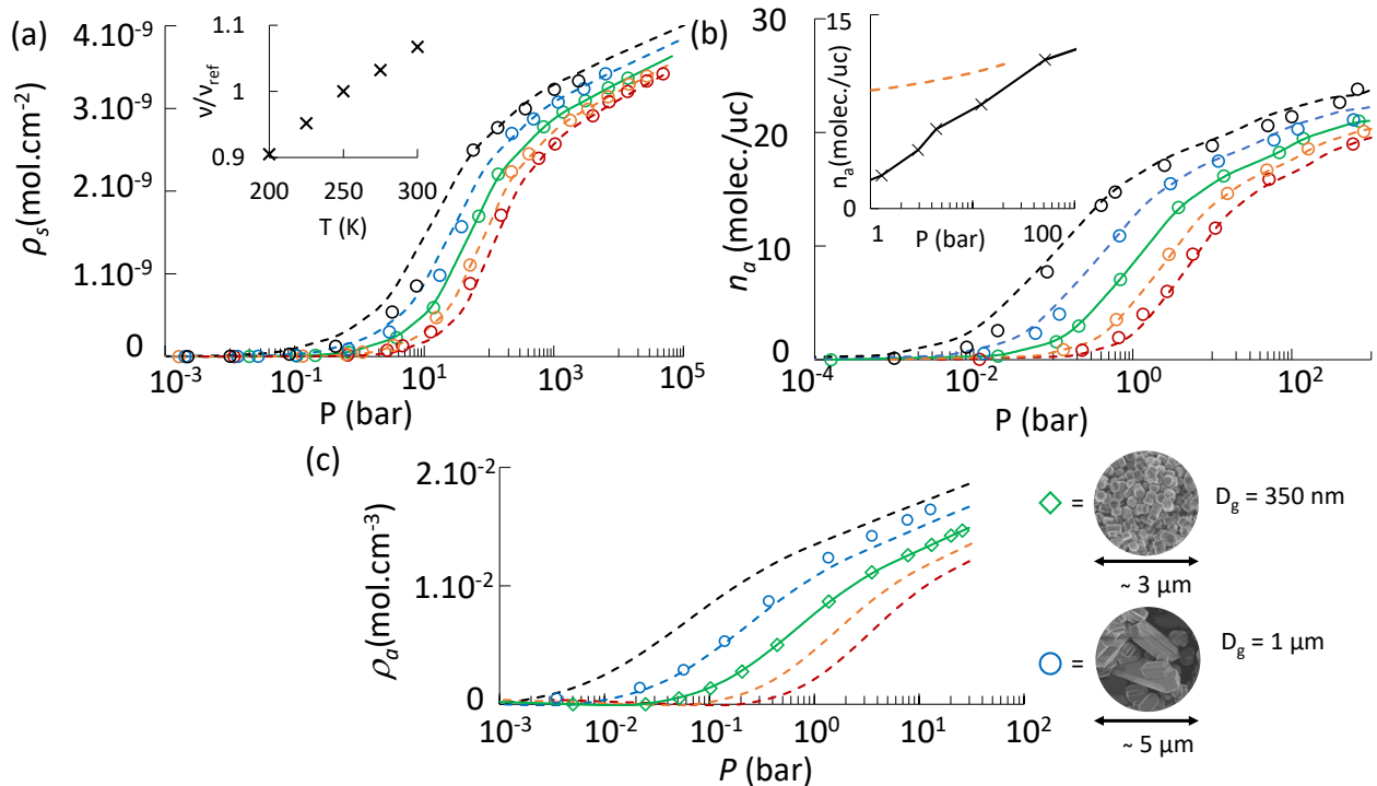
Figure 6: (color online) Polanyi's adsorption potential theory applied to simulated methane adsorption isotherms in zeolite layer a (a) and in a zeolite crystal (b) at different temperatures T . In (c), Polanyi's model is applied to our experimental data. Different colors correspond to the following temperatures: 300 K (red), 275 K (orange), 250 K (green), 225 K (blue), 200 K (black). The open symbols correspond to the simulated/experimental adsorbed amounts as obtained using Monte Carlo simulations in the Grand Canonical ensemble/adsorption volumetric technique. For the three figures, the adsorption isotherm obtained at T = 250 K (green data) was used as reference data to predict the adsorption isotherms obtained at other temperatures. The dashed lines correspond to the predictions from Polanyi's model at different temperatures T' . In (c) the adsorption isotherm for the powder of D_g = 350 nm at 250 K was used as the reference to predict the adsorption of the powder of D_g = 1 \mu\text{m} at 225 K. The adsorbed amount n_a is expressed in \text{mol}\cdot\text{cm}^{-2} (a), number of methane molecules per zeolite unit cell (b) and \text{mol}\cdot\text{cm}^{-3} (c). The insert in figure (a) corresponds to the ratio of the molar volume at T over the molar volume at the reference temperature T = 250 K. The insert in figure (b) corresponds to the adsorption data predicted using the FHH approximation in combination with the interaction potential by Peterson et al. . These data correspond to the adsorbed amount in the straight channels of silicalite-1 in the pressure range from 1 to 100 bar. The black line corresponds to the adsorption isotherm for the zeolite channels obtained by means of molecular simulation. The dashed orange line corresponds to the adsorption isotherm calculated using the attractive part of the interaction potential by Peterson et al. 58
