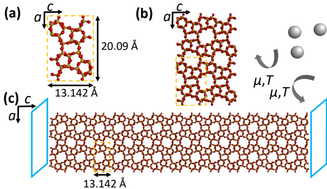
Figure 1: (color online) Silicalite-1 zeolite crystal. The Si and O atoms are represented as yellow and red spheres, respectively. a , b , c denote the crystallographic axes which are aligned with the x , y and z axes of the Cartesian reference frame. A single unit cell is represented in (a) while a 2 \times 2 \times 2 crystal is shown in (b). Periodic boundary conditions (PBC) are applied in each direction to mimic an infinitely large system and, hence, avoid finite size effects. (c) The MFI unit cell was duplicated 10 times along the chosen direction (the layer axis, here z ) and 2 times along the other directions (perpendicular to the layer axis, here x and y ) to form a zeolite layer with an external surface. Methane adsorption is simulated by setting the system in contact with a fictive bulk reservoir which imposes its temperature T and chemical potential \mu .
