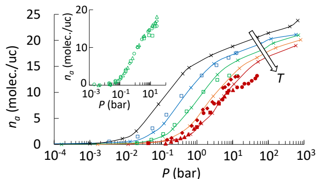
Figure 2: (color online) Experimental and simulated adsorption isotherms n_a(P) for methane at different temperatures in silicalite-1 zeolite. The different colors correspond to the following temperatures: 200 K (black), 225 K (blue), 250 K (green), 275 K (orange), 300 K (red). The lines with crosses correspond to the results from our molecular simulations. The symbols without lines correspond to experimental data. The open symbols correspond to our experimental data. The closed symbols correspond to experimental data at 300 K from other groups: Abdul-Rehman et al. (diamonds), Ding et al. (circles), Golden and Sircar (squares), Richard and Rees (triangles). All these experimental data were reproduced from Smit et al. 42 The adsorbed amount n_a is expressed in number of methane molecules per zeolite unit cell. The arrow indicates data obtained for increasing temperatures. The insert shows our experimental data obtained at 250 K for powder samples with different grain sizes: D_g = 1 \mu\text{m} (squares), 350 nm (diamonds), 200 nm (circles), 80 nm (triangles).
