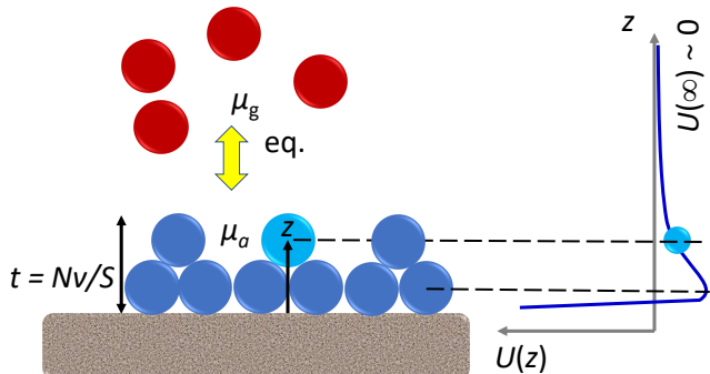
Figure 5: (color online) Schematic representation of the adsorption potential theory. The chemical potential of the fluid phase (red spheres) is \mu_g . The adsorbed phase (blue spheres) has a statistical film thickness t which can be converted from the adsorbed volume Nv as t = Nv/S where N is the number of adsorbed molecules, v the molar volume and S the surface area of the solid phase. For the adsorbed phase, the chemical potential \mu_a is described using a perturbation term by assuming that it corresponds to the chemical potential \mu_0 of the bulk liquid at saturation corrected for the interaction U(z) with the solid surface: \mu_a - \mu_0 = U(z) . At very small z , the surface interaction potential U(z) is positive due to repulsive interactions with the solid surface. At larger z , U(z) becomes negative with a minimum located at a distance corresponding approximately to the position of the first adsorbed layer. At larger z , U(z) goes to zero as interactions with the solid surface become vanishingly small.
