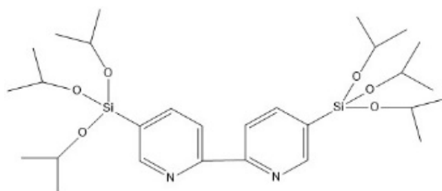
Figure 7. Chemical formula of the 5,5'-bis(triisopropoxysilyl)-2,2'-bipyridine ( i Prbipy) precursor.
