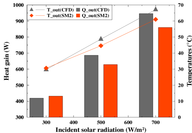
Figure 15. Variation in the temperature and heat gain of the air at the outlet with incident solar radiation.
