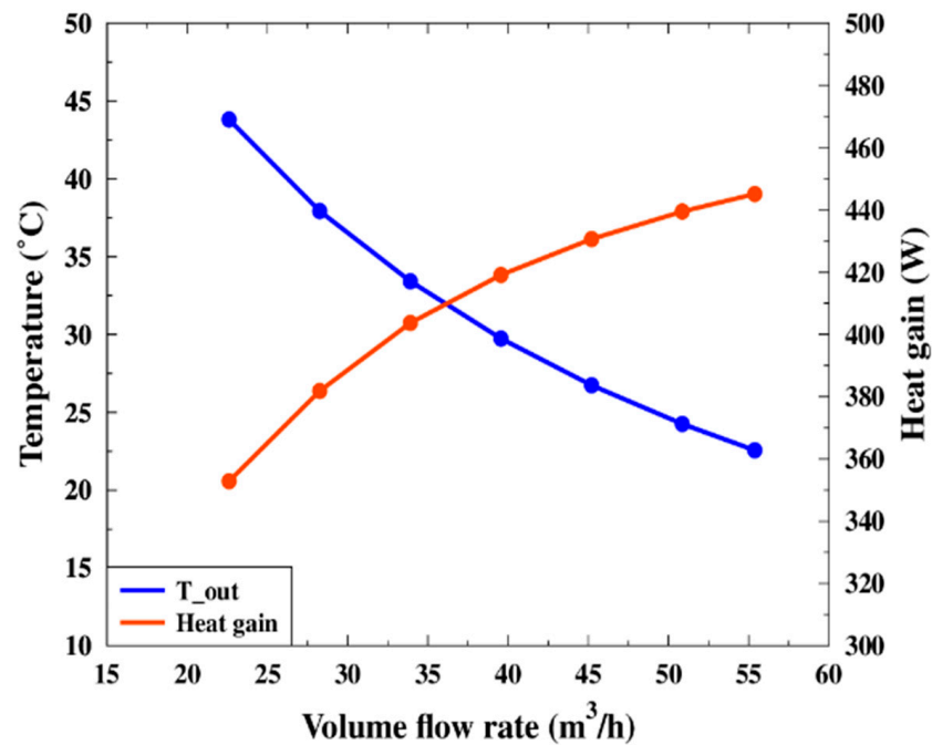
Figure 9. Variation in outlet temperature and heat gain with the imposed airflow rate.
