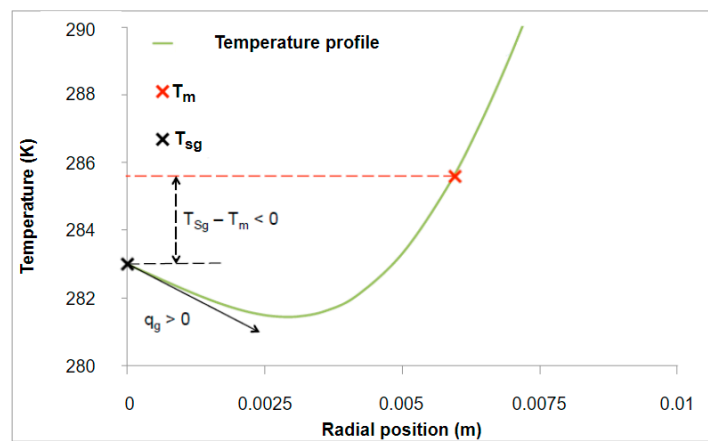
Figure 7. Temperature profile in the air gap [35]. Reprinted with permission from Ref. [35]. Copyright 2014 Gloriant, F.A.F. All rights reserved.
