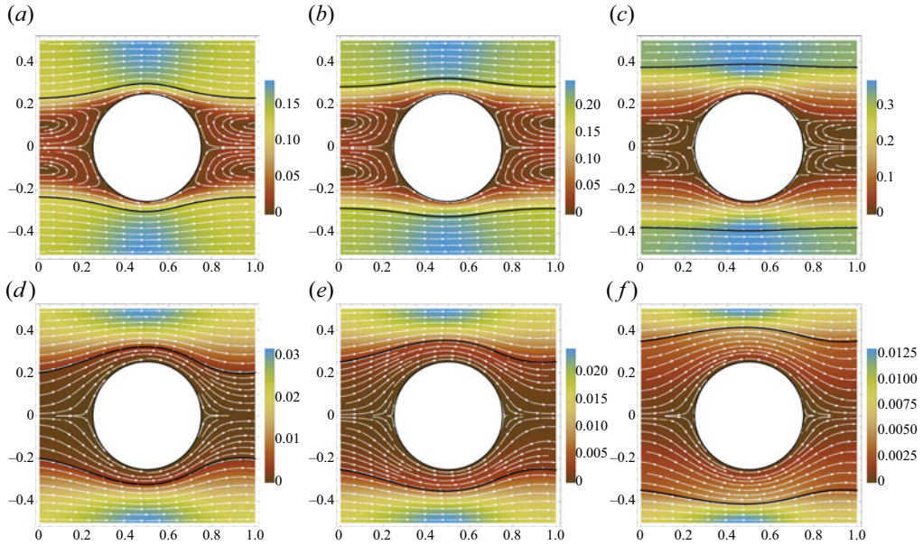
Figure 5. Unit-cell fields of the dimensionless velocity magnitude and corresponding streamlines (in white) obtained from DNS with Ca = 10 ; (a–c) \mu^* = 0.1 ; (d–f) \mu^* = 10 ; (a,d) S_\beta = 0.4 ; (b,e) S_\beta = 0.5 ; (c,f) S_\beta = 0.7 . Here \mathcal{A}_{\beta\gamma} and \mathcal{A}_{\beta\sigma} are shown by black lines; \varepsilon = 0.8 .
