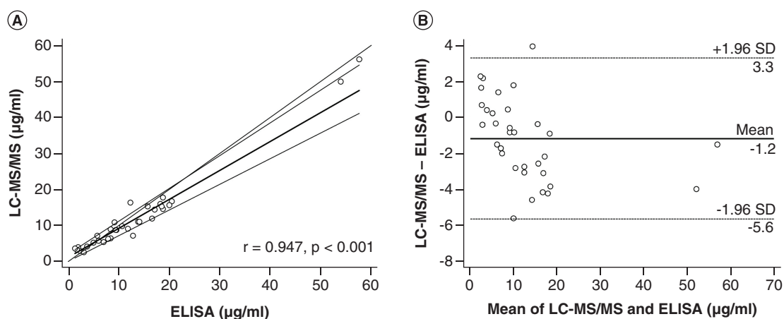
Figure 3. Methods comparisons for adalimumab. (A) Passing–Bablok regression plot of adalimumab concentrations measured by LC-MS/MS and in-house ELISA in samples from patients with inflammatory bowel diseases treated with Adalimumab ( n = 34 ). (B) Bland–Altman analysis of the difference between LC-MS/MS and in-house ELISA. The mean \pm 2 standard deviation lines (95% limits of agreement) are plotted for reference.
