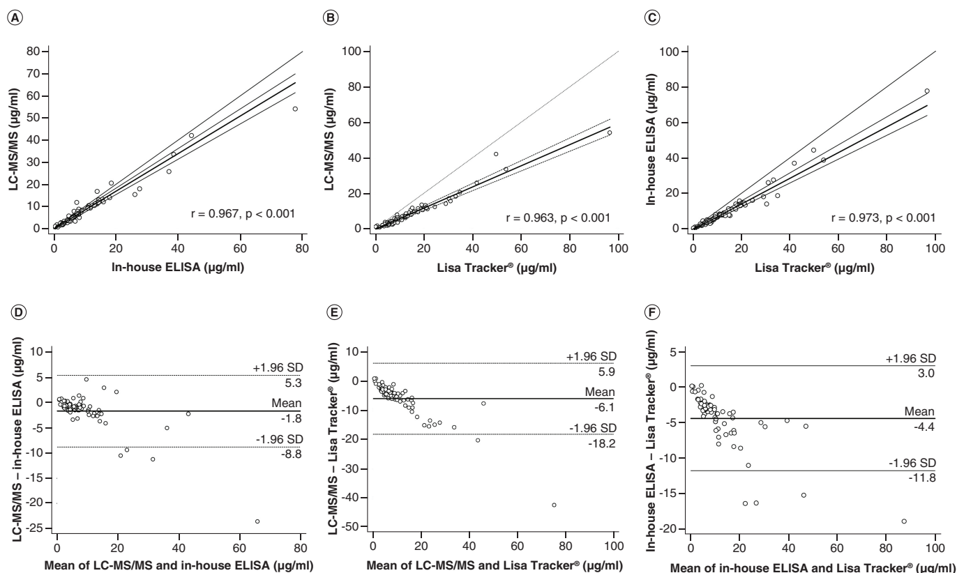
Figure 2. Methods comparisons for infliximab. Passing-Bablok regression plot of infliximab concentrations as measured by (A) LC-MS/MS and in-house ELISA, (B) LC-MS/MS and the commercial Lisa-Tracker® kit, (C) in-house ELISA and the commercial Lisa-Tracker® kit. Concentrations were measured in samples from patients with inflammatory bowel disease treated with IFX (n = 70). Bland-Altman analysis of the difference between (D) LC-MS/MS and in-house ELISA, (E) LC-MS/MS and the commercial Lisa-Tracker® kit, (F) in-house ELISA and the commercial Lisa-Tracker® kit. The mean ±2 standard deviation lines (95% limits of agreement) are plotted for reference. ELISA: Enzyme-linked immunosorbent assay; LC-MS/MS: Liquid chromatography tandem mass spectrometry.
