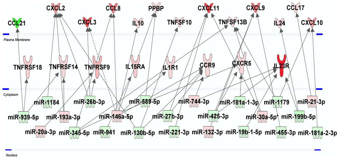
FIGURE 4 | miRNA-mRNA networks generated with Ingenuity Pathway Analysis (IPA) for H37Rv-infected human macrophages. IPA analysis was performed to investigate the connection between the 30 and 37 H37Rv-specific host inflammatory response gene set and miRNAs, respectively. Filters were set to only include experimentally observed or high-confidence-predicted miRNA-mRNA interaction partners. Genes and miRNAs were colored in red or green depending on whether they were upregulated or downregulated (respectively) with respect to their uninfected controls and the shading intensity shows to what degree each miRNA or gene was deregulated. Direct and indirect miRNA-gene interactions are represented with a solid and dotted lines, respectively.
