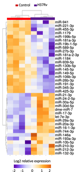
FIGURE 3 | Expression levels of miRNAs significantly deregulated after H37Rv infection. THP-1 differentiated into macrophages were infected with H37Rv for 48 hours ( n = 4 ). After total RNA including small RNA extraction, the expression level quantification of 762 human miRNAs was performed using TaqMan ® Array Human MicroRNA Card. Using Clustvis software, a supervised hierarchical analysis of the distribution of macrophage samples based on relative log2 expression of 37 miRNAs significantly modified by H37Rv infection compared to uninfected controls. Statistical analysis was performed on \Delta Ct using Student's t test to identify the differently expressed miRNAs compared with uninfected controls. Imputation was used for missing value estimation. Samples were clustered using the correlation distance method and average linkage.
