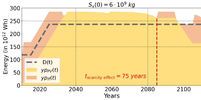
Fig. 5. Energy mix of France following the scenario B with S_x(0) = 6 billion kilograms and t_f = 100 years. Highlighting the scarcity effect on the PV production after 75 years.
