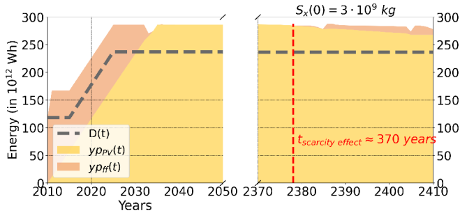
Fig. 9. Energy mix of France following the scenario C with t_f = 400 years and S_x(0) = 3 billion kilograms. Highlighting of delayed scarcity effect.
