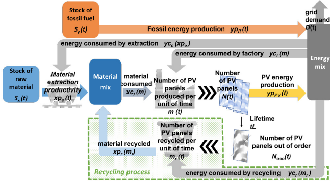
Fig. 1. Modular diagram representing interactions between PV panels factory, matter and energy stocks, and energy mix. The recycling module is surrounded in a green frame, its implementation depends on the chosen scenario to run. Same for grid energy demand D(t) .
