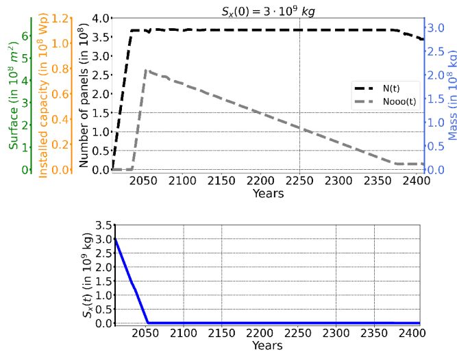
Fig. 10. Number of panels (up part), produced (dashed black line) and out of order panels (dashed gray line) following scenario C with t_f = 400 years and S_x(0) = 3 billion kilograms. Raw material stock as a function of time (bottom part, blue line). Highlighting of the two steps leading to scarcity effect after 370 years.
