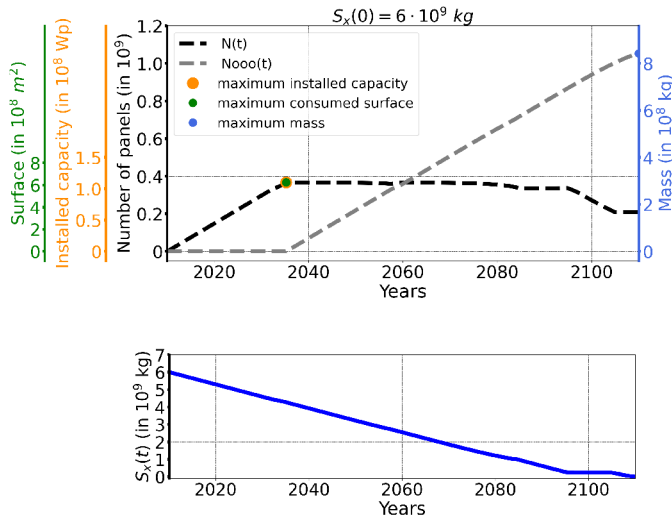
Fig. 6. Operational panels (black dashed line) and out of order panels (gray dashed line) (up), and stock of raw material (blue line) as functions of time, following the scenario B with S_x(0) = 6 billion kilograms. and t_f = 100 years.
