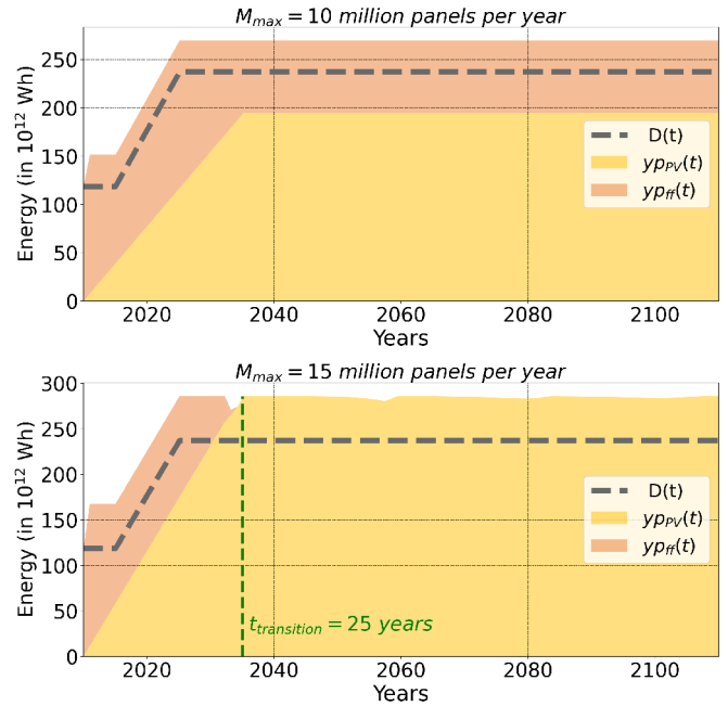
Fig. 3. Energy mix of France following the scenario A over 100 years, varying limitation of factory productivity M_{\max} , from 1 \times 10^7 (upper) to 1.5 \times 10^7 (lower) panels per year. Fossil fuel production (in orange), PV production (in yellow) and grid energy demand (dashed black line). Transition date t_{\text{transition}} (in green) pinpoints when a 100% PV energy mix is reached.
