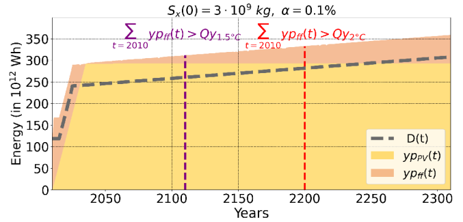
Fig. 11. French energy mix following the scenario D, with t_f = 400 years and with S_x(0) = 3 billion kilograms. Purple and red vertical dashed lines respectively define dates, 2110 and 2200, for which total fossil fuel consumption overtakes power generation carbon budget of France to maintain global warming below 1.5 and 2 °C.
