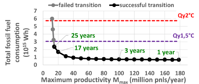
Fig. 4. Total fossil fuel consumption of runs with varying maximum productivity M_{\max} , with t_f = 100 years. Each dot corresponds to a run with a specific M_{\max} . Gray and black dots correspond respectively to failed and successful energy transition along with its duration (in green). Dashed lines represent power generation carbon budget of France to maintain global warming below 1.5^\circ\text{C} (in purple) and 2^\circ\text{C} (in red).
