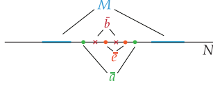
Figure 6: The structures M < N , a set B and two tuples, \bar{a}, \bar{e} , with \bar{a} \downarrow_M B and \bar{e} \not\downarrow_M B .
