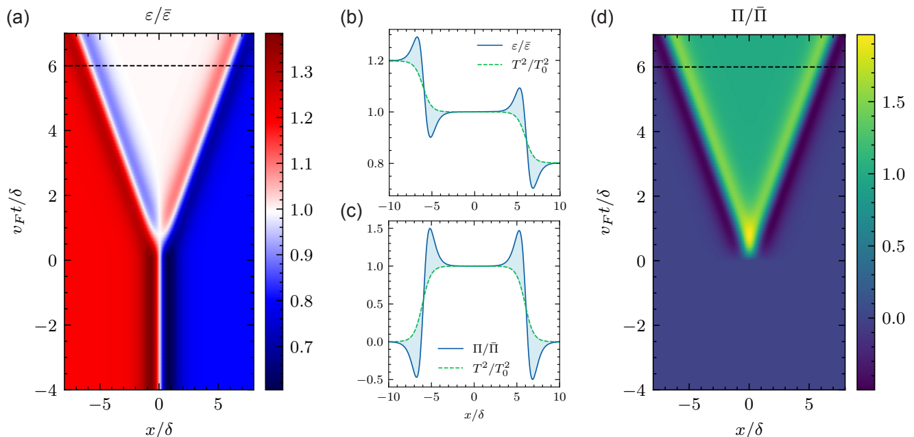
Figure 5. Quantum corrections to energy traveling waves imposed by a temperature quench. (a) Two halves of a wire of non-interacting particles ( c_+ = c_- = 1 ) with Fermi velocity of v_F = 10^6 \text{ ms}^{-1} are set at two temperatures T_{R/L} = T_0 \pm \Delta T/2 following the same protocol as in Fig. 3. The average temperature is T_0 = 100\text{mK} , and the ramp of temperature of amplitude \Delta T = 20\text{mK} is imposed over a length \delta = 10\mu\text{m} . At time t = 0 this external temperature difference is released. Following this quench, two traveling waves of energy appear. (b) The non-monotonous behavior of the density of energy profile is a manifestation of the anomaly corrections originating from quantum fluctuations of similar nature than close to a black hole. The amplitude of the corrections, represented by the shaded area, is a direct measure of the new quantum scale of energy \varepsilon_q^{(1)} \simeq \varepsilon_q^{(2)} set by gravitational anomalies. In between the two waves, appears a region of homogeneous density of energy \bar{\varepsilon} = \frac{1}{2}\gamma(c_+ T_L^2 + c_- T_R^2) = \gamma(T_0^2 + \Delta T^2) . (c) and (d) This intermediate region is not in equilibrium: it is crossed by right moving particles at temperature T_L and left moving particles at temperature T_R , leading to a steady current \bar{J}_\varepsilon = \frac{1}{2}\gamma v_F (c_+ T_L^2 - c_- T_R^2) = 2\gamma v_F T_0 \Delta T and momentum \bar{\Pi} = v_F^{-2} \bar{J}_\varepsilon . The oscillating corrections to the momentum or energy current close to the interface between the three regions, shown in (b) and (c) as shaded areas, are also an accessible manifestation of corrections due to quantum fluctuations due to the trace and gravitational anomalies, similarly to those at the vicinity of a black hole. In the present case they originate from the local strong curvature of the effective spacetime accounting, following Luttinger equivalence, for the temperature variation.
