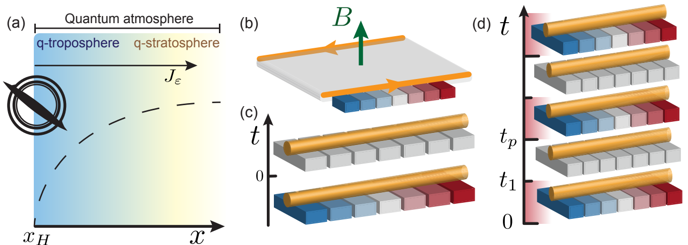
Figure 1. Four situations considered in this work where gravitational anomalies play a role through the anomalous Tolman-Ehrenfest temperature. (a) A black-hole’s Hawking temperature at spatial infinity is fixed by an outgoing heat current J_\epsilon is determined by the gravitational anomalies: it originates from strong quantum fluctuations in a region close to the the horizon ( x_H ), a quantum atmosphere. (b) The edge of a 2D quantum Hall system hosts a 1+1 dimensional chiral edge mode. The difference between an externally imposed temperature profile, and the equilibrium temperature of the edge-mode is set by the anomalous Tolman-Ehrenfest temperature. (c) A quantum wire undergoes a quantum quench when an external temperature profile is suddenly switched off at time t = 0 . The energy density profile following this quench displays oscillating features determined by gravitational anomalies. (d) A periodic dynamic is implemented by repeating over a period t_p the previous thermal quench procedure. Within a heating phase, the energy density of the quantum wire increases exponentially, showing imprints of gravitational anomalies at spatially localized at points acting as black-hole analogues.
