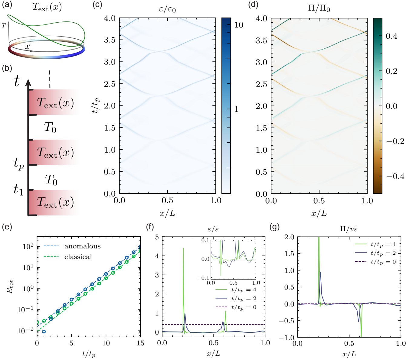
Figure 6. Floquet heating state. (a) We consider a ring of free relativistic fermions of velocity v_F = 1 . (b) This ring is driven periodically by an external temperature with a period t_p = t_1 + t_2 , such that (i) during time t_1 the external temperature is a smooth profile T_{\text{ext}}(x) varying around an average T_0 , shown in (a), and (ii) during time t_2 temperature is kept to a constant T_0 . The two times Lt_1/v_F = 0.1 and Lt_2/v_F = 0.45 , are chosen such that the period coincides with the time of flight of particles around the ring: L = v_F t_1 + \tilde{v}_F t_2 where \tilde{v}_F is the averaged effective velocity under the temperature profile T_{\text{ext}}(x) . (c) and (d) As a function of time, both the energy density \varepsilon and the momentum \Pi become highly inhomogeneous, and concentrate on a few trajectories. They are represented rescaled by the classical values \varepsilon_0 = v_F \Pi_0 = \gamma T_0^2 . The energy and momentum profiles are represented after two and four periods in panels (f) and (g), illustrating the localization mechanism. (e) Besides being focused spatially, the net energy of the ring E_{\text{tot}} = \int_0^L \varepsilon dx = L\bar{\varepsilon} increases: the Floquet state is heating. This is represented by monitoring the stroboscopic dynamics at times t_n = nt_p of the ring for which E_{\text{tot}} increases exponentially. Remarkably the rate of increase of this energy is not classical: quantum fluctuations, responsible for the trace and gravitational anomaly corrections, have a growing energy. The two focusing trajectories behave as heating black holes: in their neighborhood the energy density becomes negative, as shown in the inset of panel (f). This is an additional manifestation of the effects of quantum fluctuations induced by a local large curvature similar to those in a black-hole atmosphere.
