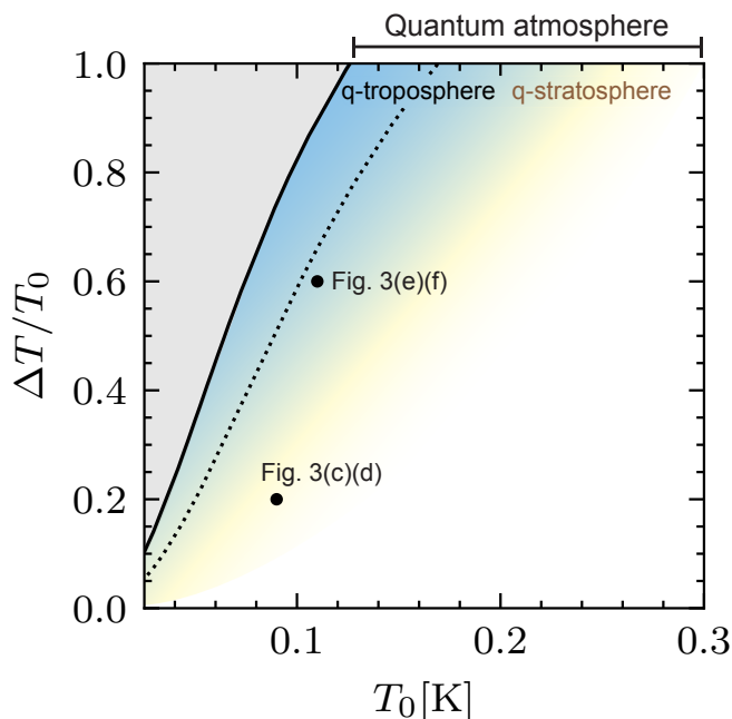
Figure 4. Diagram of the possible out of equilibrium thermodynamic states imposed by a temperature jump. The phase diagram corresponds to an imposed temperature profile, as represented in Fig. 3(b), varying between two temperatures T_{R/L} = T_0 \pm \Delta T/2 over a length \delta = 10 \mu\text{m} . The white region corresponds to the region with classical fluctuations where gravitational anomalies can be neglected. As in Fig. 2, the colored region signals the quantum atmosphere, and the color encodes the smooth crossover between the quantum stratosphere, where \varepsilon_q = \varepsilon_q^{(1)} \approx \varepsilon_q^{(2)} , and the quantum troposphere, where \varepsilon_q^{(1)} \neq \varepsilon_q^{(2)} . The relevance of quantum fluctuations is signaled by the relation \lambda_T(x) \gtrsim l_T(x) close to the temperature jump, between the thermal length \lambda_T and l_T = |\partial_x^2 T/T|^{-1/2} which characterises the temperature variation. The quantum troposphere is characterized by an additional length scale l_T^{(2)} = |\partial_x T/T|^{-1} \neq l_T defined by the imposed temperature profile. As in Fig. 2(a) the dotted line represents the state possessing black hole like thermodynamic local properties ( \varepsilon < 0 but T_{eq}^2 > 0 ). The thermodynamically forbidden region, in which the \varepsilon + P and the entropy are negative and our extended Luttinger correspondence does not apply, is shaded in gray. The two black dots represent the parameters chosen for Fig. 3. We chose the Fermi velocity to be v_F = 10^6 \text{ m} \cdot \text{s}^{-1} , typical for relativistic materials.
