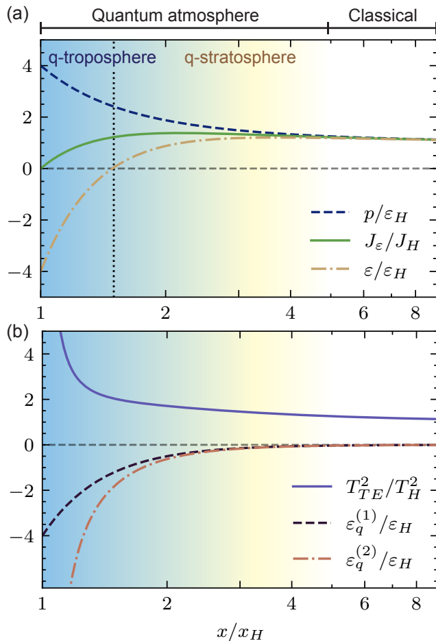
Figure 2. Quantum atmosphere of a D = 1+1 Schwarzschild black hole. (a) the dimensionless energy density \varepsilon , pressure p and energy current J_\varepsilon , rescaled by their asymptotic values \varepsilon_H = \frac{1}{2}\gamma T_H^2 and J_H = (\pi/12\hbar)k_B^2 T_H^2 where T_H is the Hawking temperature, are represented as a function of the distance x to the horizon x_H . Far from the horizon, all three quantities are proportional to T_{\text{TE}}^2(x) , where T_{\text{TE}}(x) is the classical Tolman-Ehrenfest equilibrium temperature. Close to the horizon, quantum fluctuations strongly affect this classical behavior: an anomalous equilibrium temperature T^2(x) is set by both \varepsilon + p and J_\varepsilon . (b) The difference between the anomalous T^2(x) and the classical T_{\text{TE}}^2(x) is set by a quantum scale \varepsilon_q^{(2)} . The divergence of T_{\text{TE}}^2 at the horizon is counterbalanced by a diverging correction \varepsilon_q^{(2)} , leading to a vanishing T^2(x) . Simultaneously, the difference \varepsilon_q^{(1)} between \varepsilon and p sets an independent quantum scale which remains finite at the horizon. These results illustrate the generation by a large space-time curvature R of a finite density of energy and asymptotic energy currents, which are captured by the trace and gravitational anomaly corrections to the thermodynamic quantities. In (a) and (b) The region where T^2(x) \neq T_{\text{TE}}^2(x) defines the quantum atmosphere. Within it, we defined the quantum stratosphere, where \varepsilon_q^{(1)} \approx \varepsilon_q^{(2)} , and the quantum troposphere, where \varepsilon_q^{(1)} \neq \varepsilon_q^{(2)} , color-coding the smooth crossover between them. The vertical dotted line in (a) indicates where \varepsilon = 0 .
