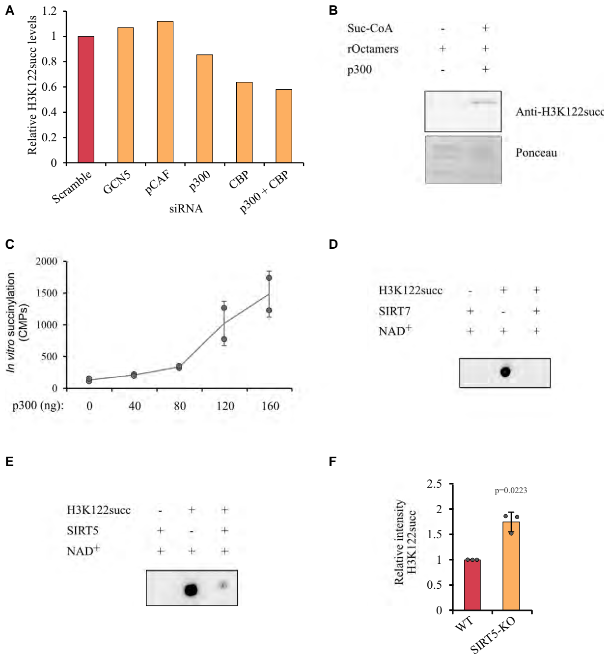
Figure 3. p300/ CBP can succinylate H3K122, SIRT5 and SIRT7 desuccinylate it.
