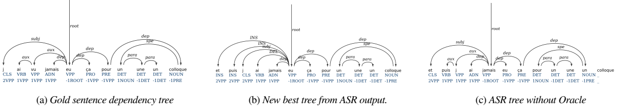
Figure 3: An example of the tree produced by the oracle with the relative encoding labeling.
