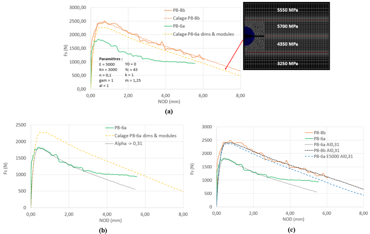
FIG. 5 - Influence of shear parameters on the fits of P8-8b and P8-6a tests with Viscohinte
