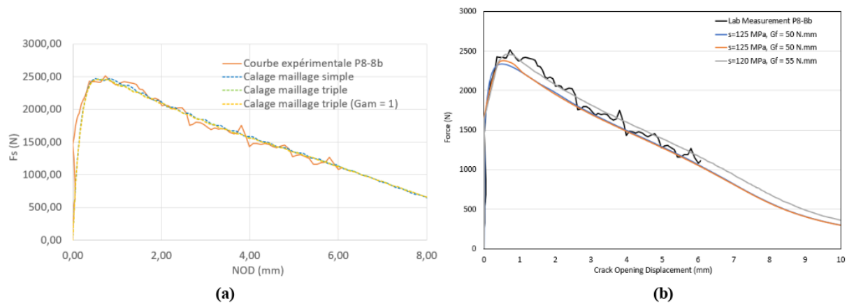
FIG. 4 - Fit of P8-8b experimental curve with (a) Viscohinte model (b) Bilinear model
