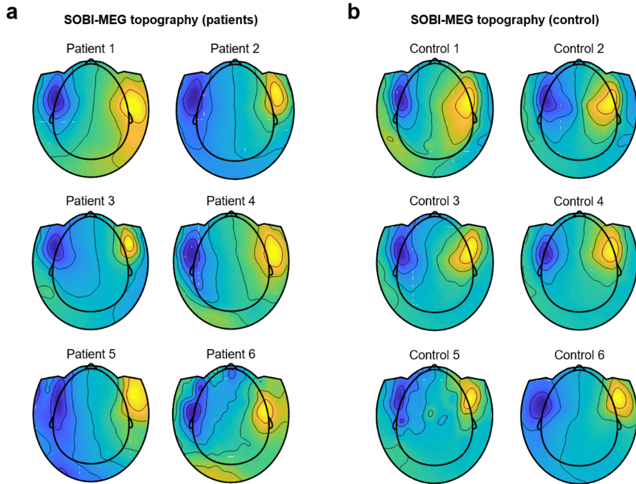
Figure 1: Second-Order Blind Identification (SOBI) magneto encephalographic (MEG) component of a putative deep source.
