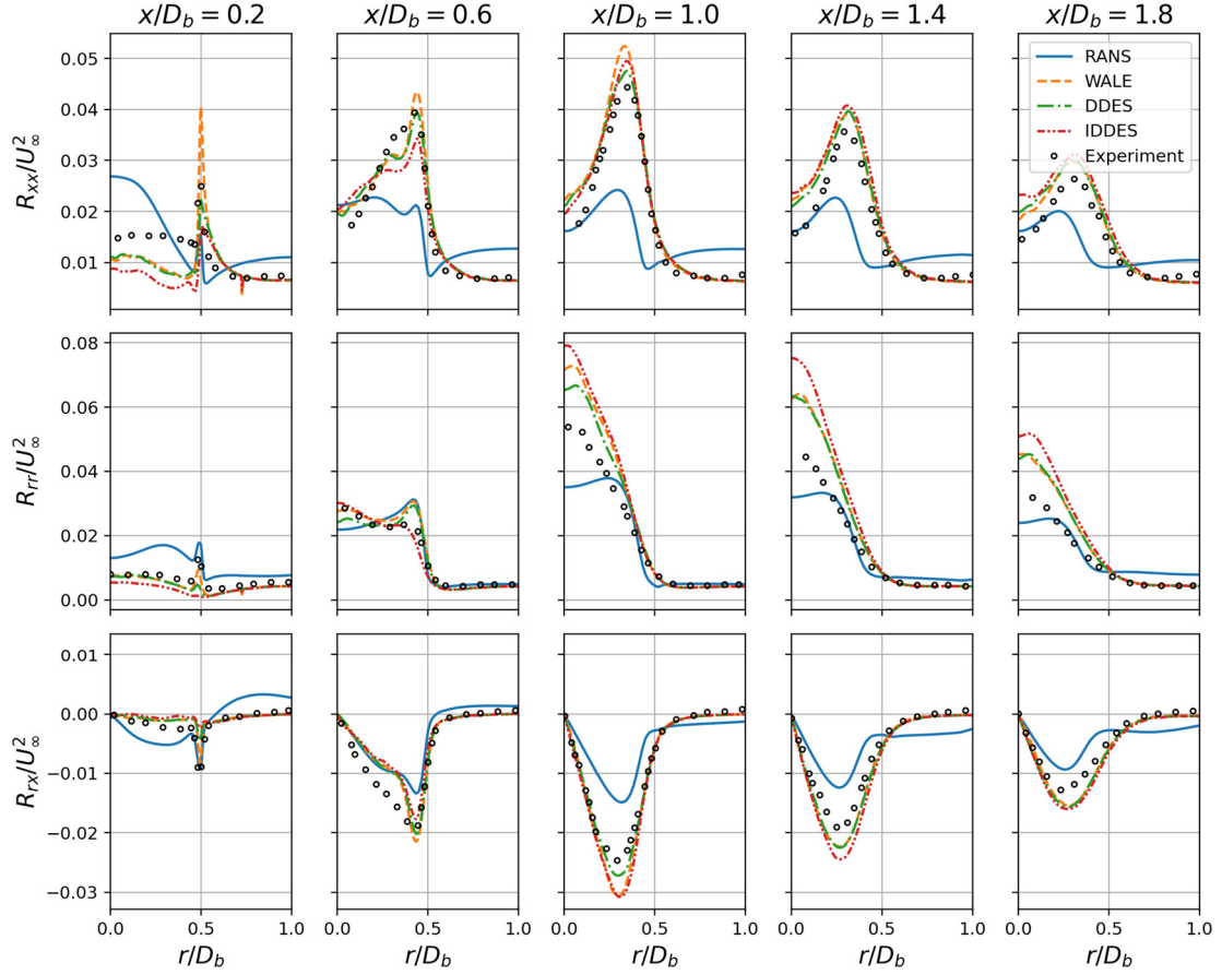
Fig. 9 Streamwise ( top ), radial ( middle ) Reynolds normal stresses, R_{xx}/U_\infty^2 and R_{rr}/U_\infty^2 respectively, and streamwise-radial ( bottom ) shear component R_{rx}/U_\infty^2 . Radial profiles evaluated at five different axial positions obtained using RANS, WALE, DDES and IDDES and compared to the corresponding experimental ones. Experiments: symbols. Numerical: lines. x/D_b is the non-dimensional axial distance.
