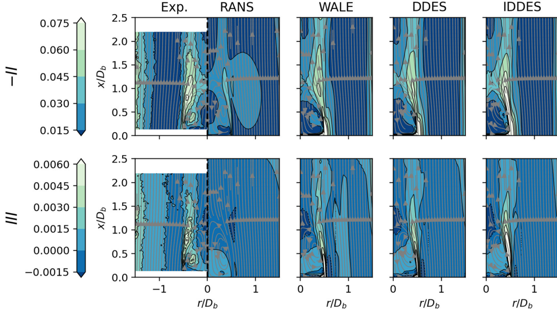
Fig. 11 Normalized anisotropy tensor second, -II , and third, III , contours of the experimental, RANS, WALE, DDES and IDDES results.
