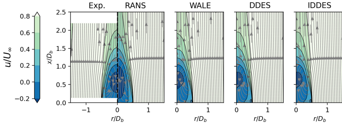
Fig. 4 Mean streamwise velocity u/U_\infty contours and streamlines of the experimental, RANS, WALE, DDES and IDDES results.
