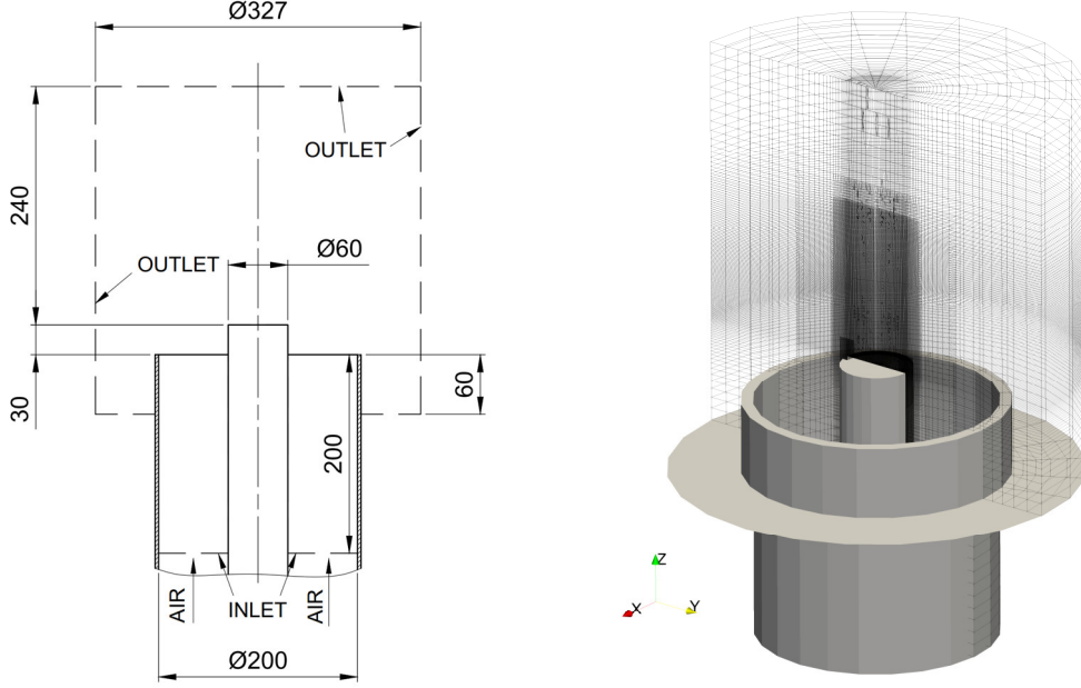
Fig. 1 Geometric configuration and computational domain ( left ), dimensions in mm. Computational mesh 3D cross-section ( right ).
