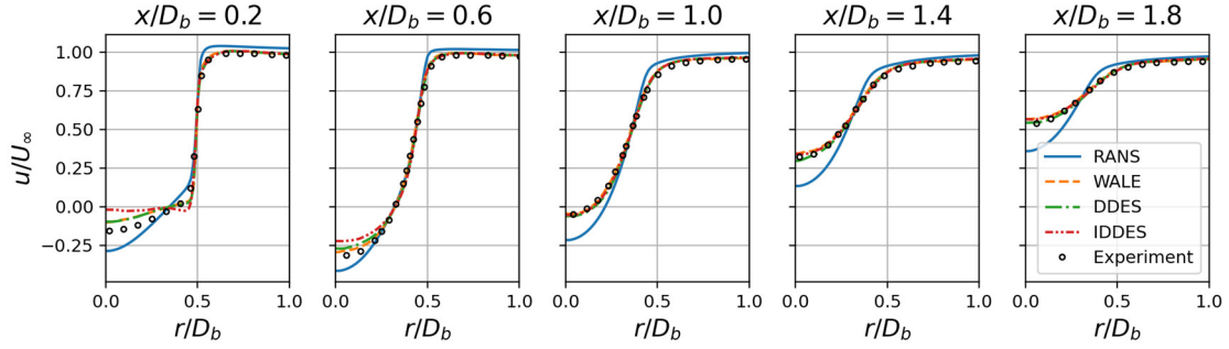
Fig. 5 Mean streamwise velocity u/U_\infty radial profiles at five different axial positions.
