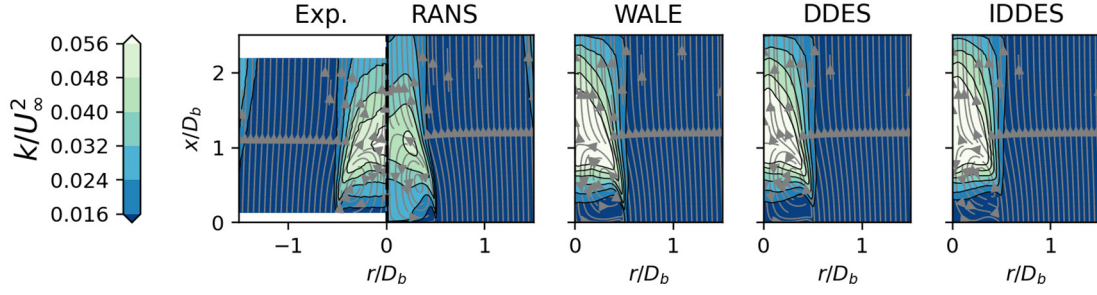
Fig. 8 Turbulent kinetic energy k/U_\infty^2 contours and streamlines of the experimental, RANS, WALE, DDES and IDDES results.
